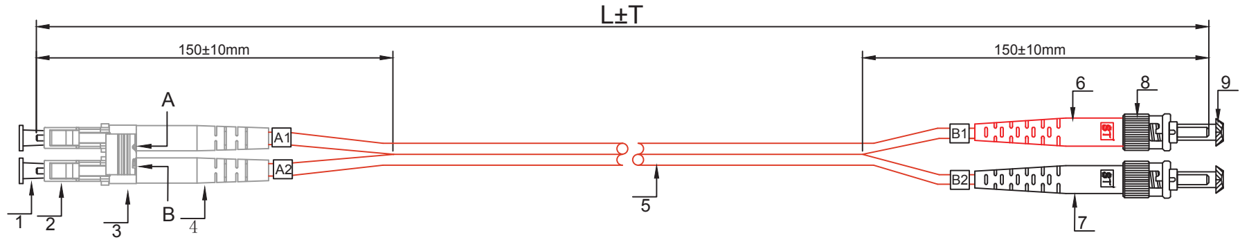
Cable Profile View
