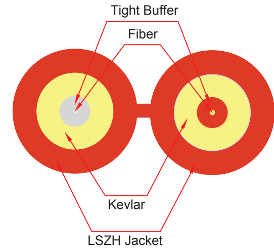
Cable Profile View
