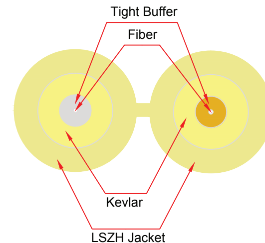
Cable Profile View
