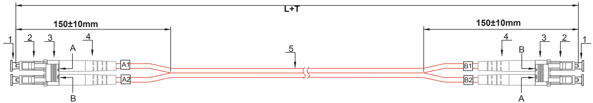
Cable Profile View
