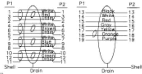
PIN Assignment
