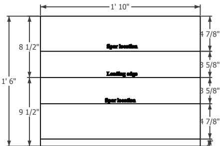
Middle section of wing
