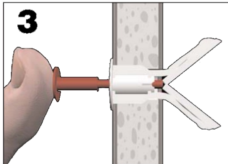
Insert anchor in hole and tap flush
