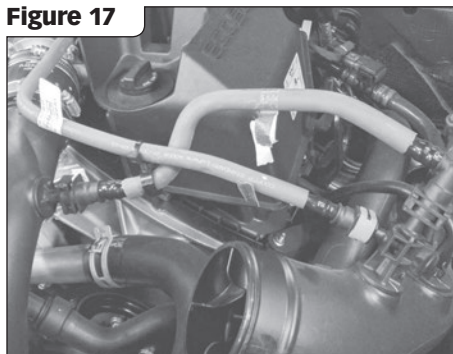
Rerouted Configuration
