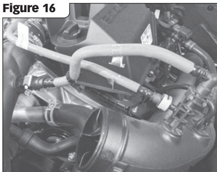
OEM Hose Configuration
