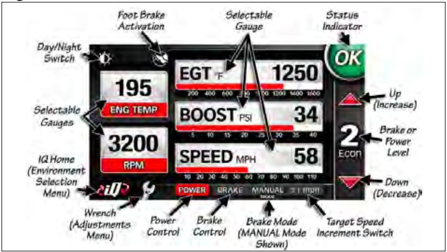
Figure 10 Combo Tuner and Brake Screen Shown.
