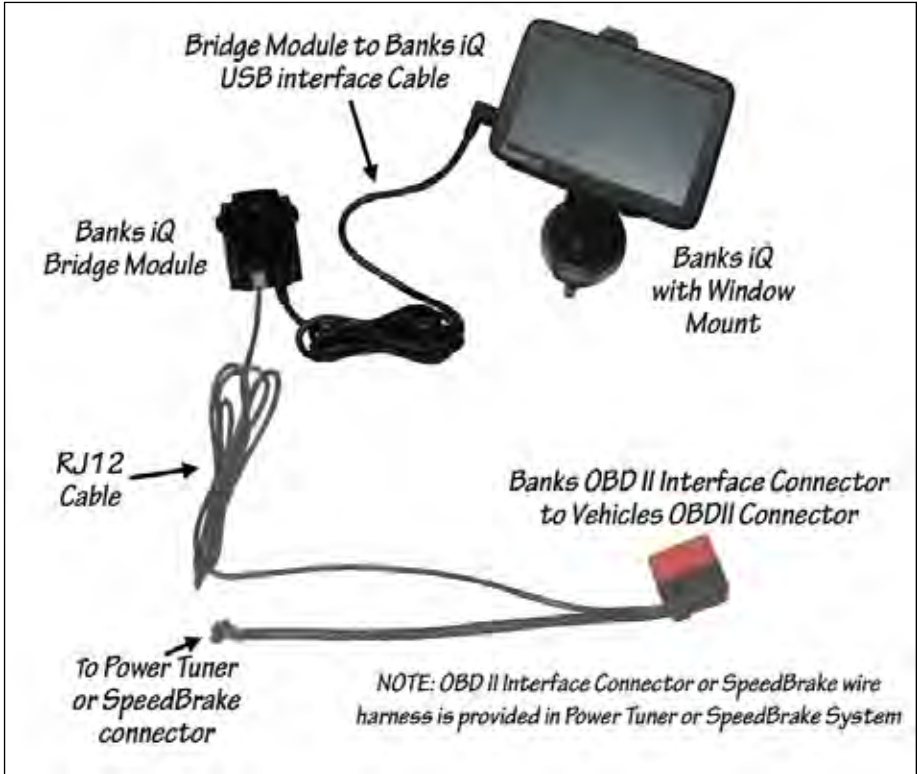
Figure 6 Banks Bridge Module
