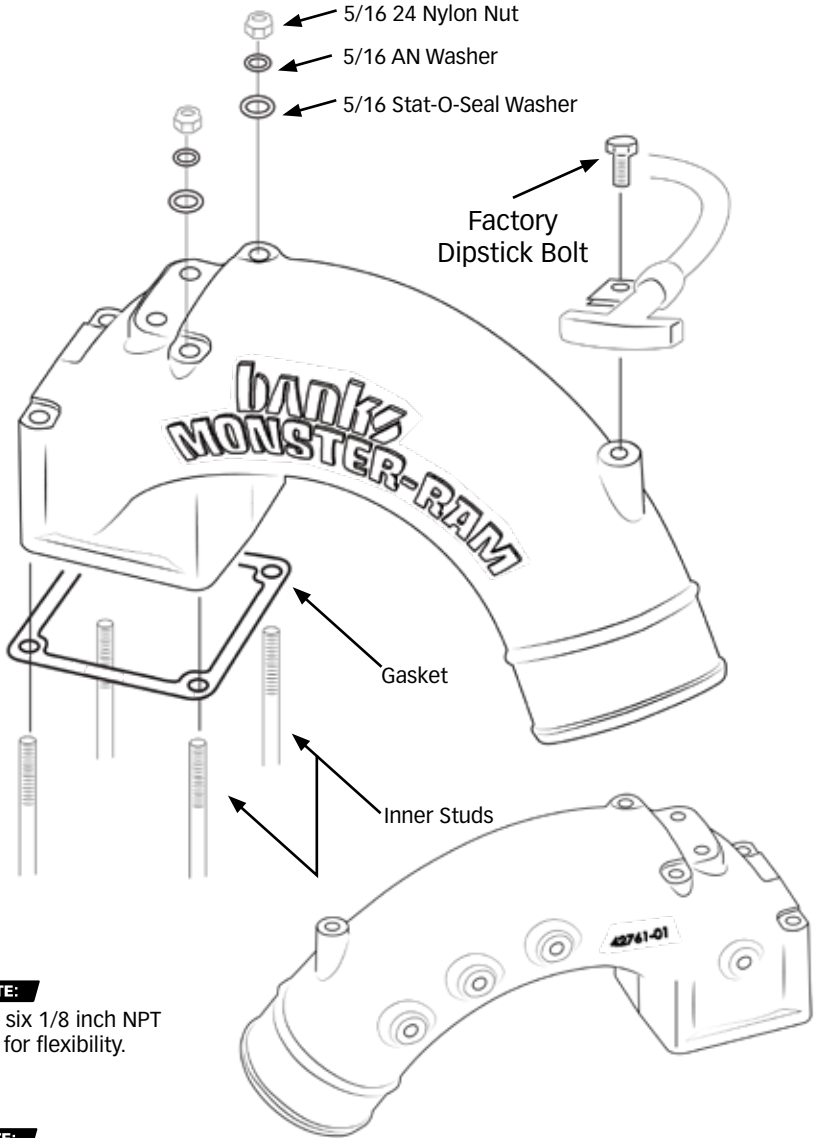
Figure 4. Exploded view of the Monster-Ram assembly
