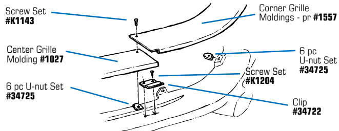
#1745 1963-64 Grille
