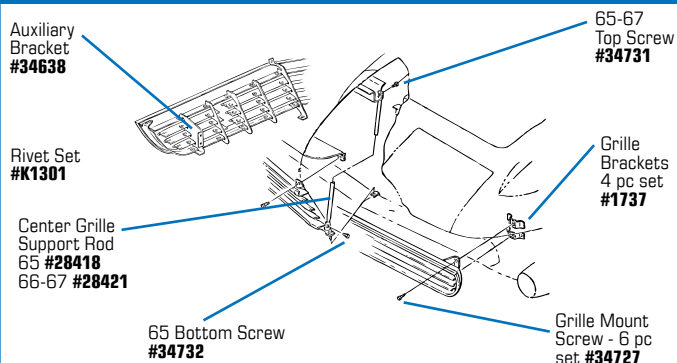
#1751 1965 Grille
