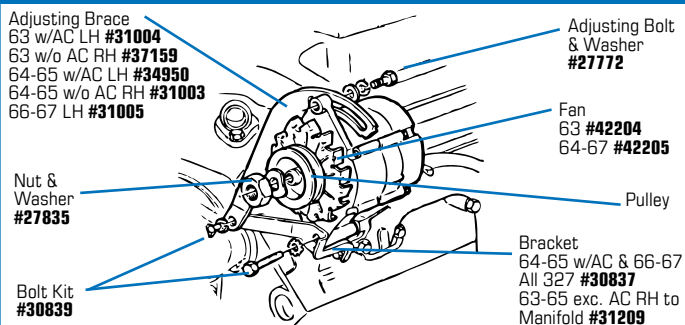
#30845 1963-67 Alternator Pulley
