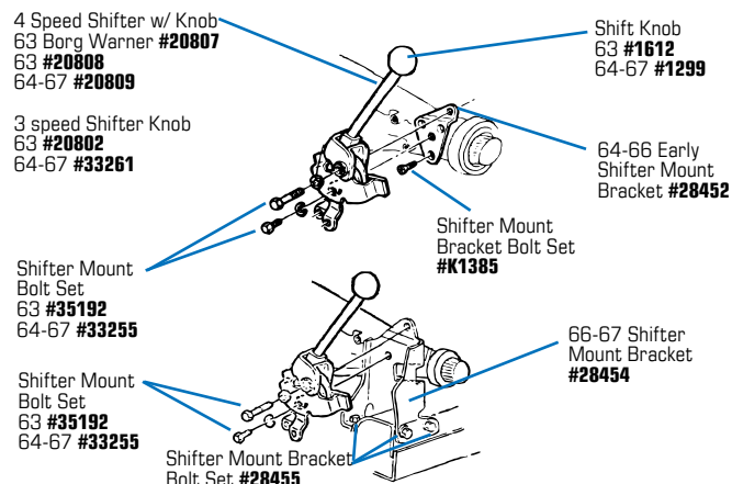
#20809 1964-67 4 Speed Shifter
