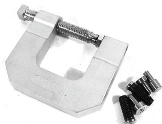
#34346 Aero-Rivet Tool
