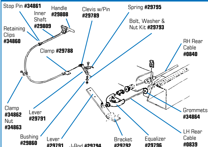
#36369 1965-66 Stainless Steel Park Brake Rebuild Kit
