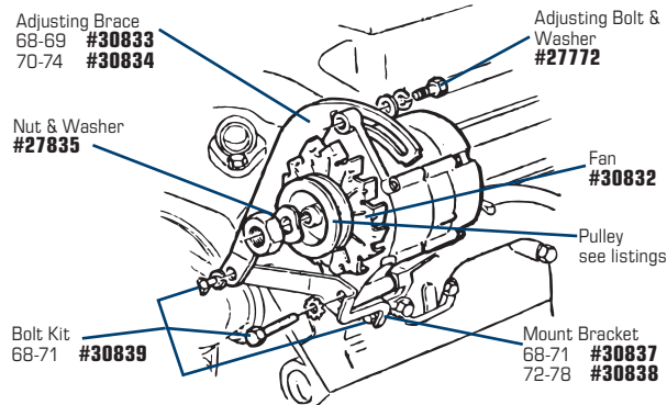
#40900 1975-78 Alternator - 78 Amp - Remanufactured
