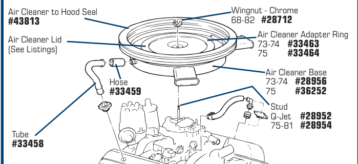
#43813 1973-75 Air Cleaner Hood Seal
