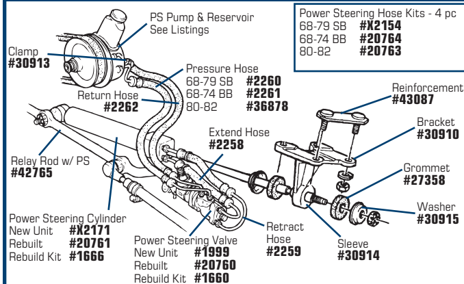
#X2171 1968-82 Power Steering Cylinder
