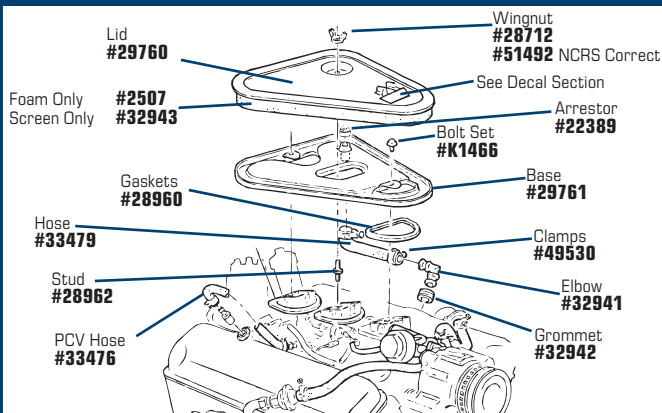
#50453 1968-72 Air Cleaner - Super Flow - 14"
