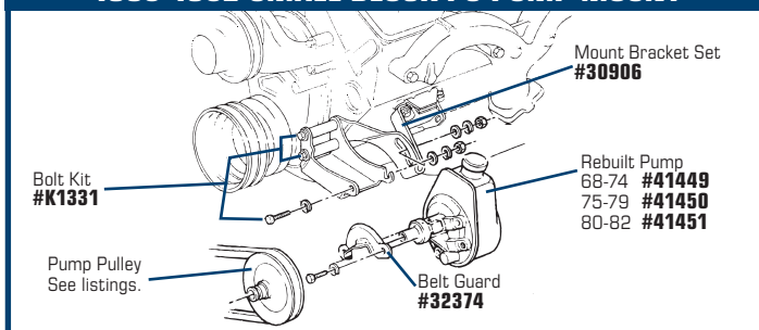
#41449 1968-74 Rebuilt PS Pump
