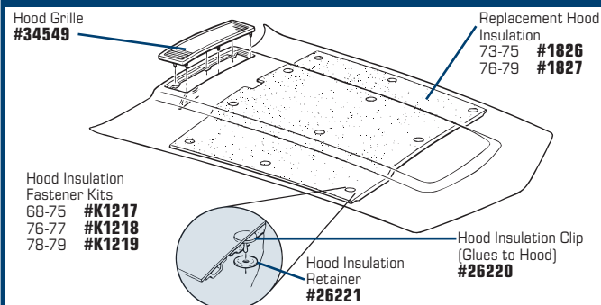
#1827 1976-79 Replacement Hood insulation
