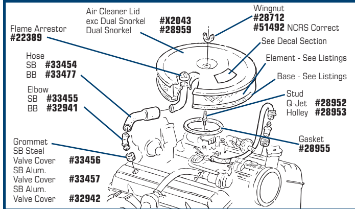
#51492 1968-72 Air Cleaner Wingnut - NCRS Correct
