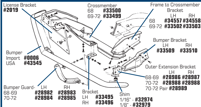
#43545 1968-72 Front Bumper - USA
