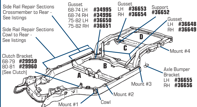
#36648 1969-1982 Frame Gussett #3 to Kickup - LH
