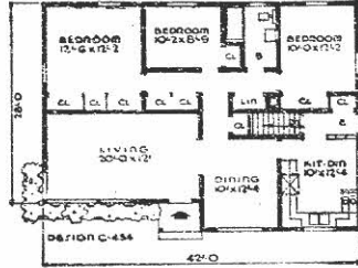
A SMALL HOUSE PLANNING BUREAU DESIGN NO. C-434
