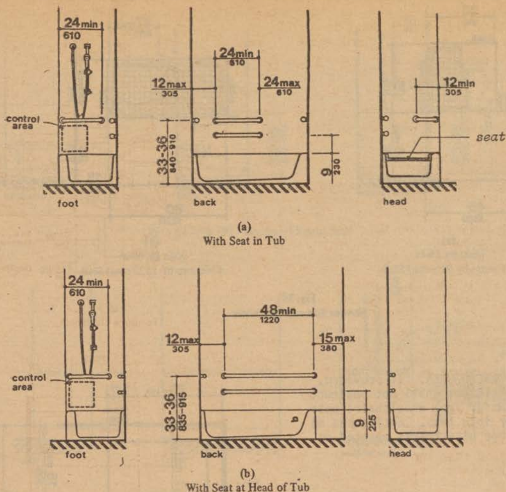
Fig. 34 Grab Bars at Bathtubs
