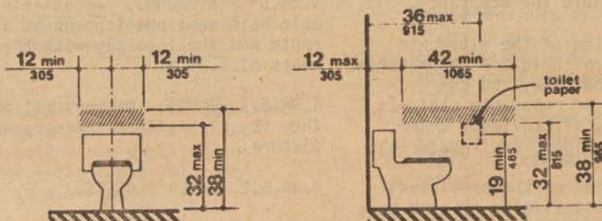
(b) Reinforced Areas for Installation of Grab Bars
