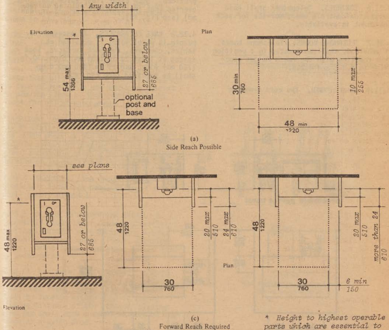
Fig. 44 Mounting Heights and Clearances for Telephones
