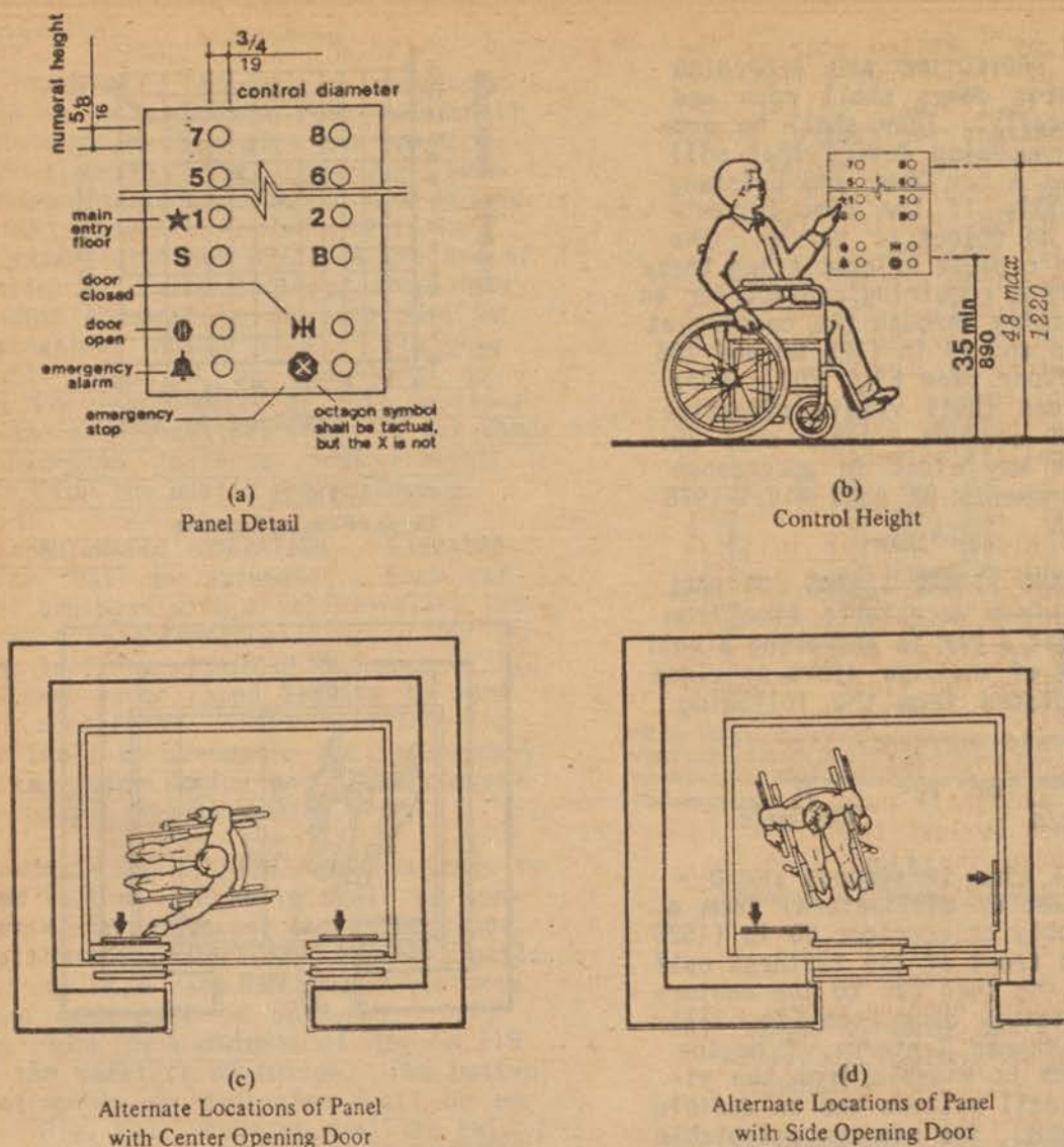
Fig. 23 Car Controls
