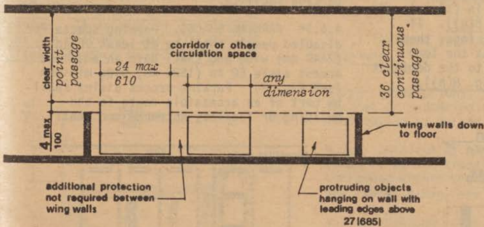
Example of Protection around Wall-Mounted Objects and Measurements of Clear Widths
