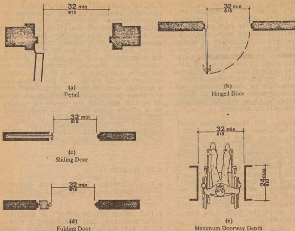
Fig. 24 Clear Doorway Width and Depth
