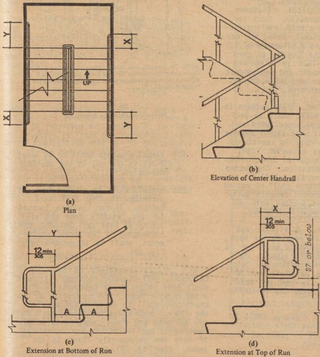
Fig. 19 Stair Handrails
