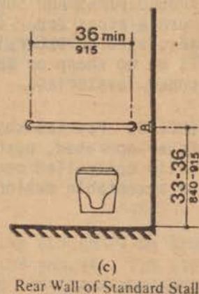
Rear Wall of Standard Stall
