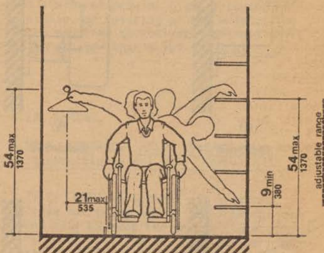
Fig. 38 Storage Shelves and Closets
