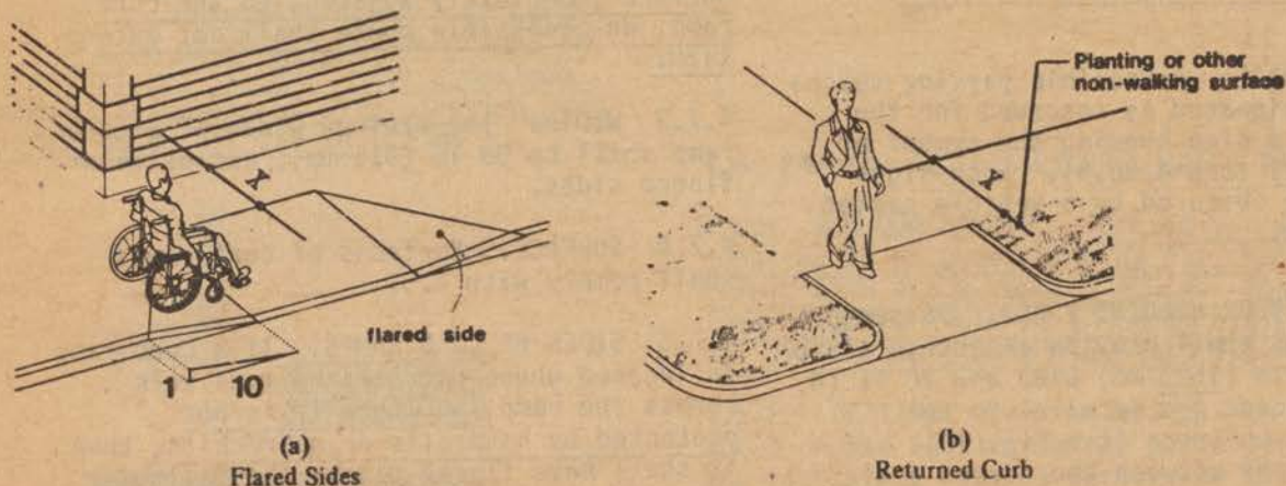
Fig. 12 Sides of Curb Ramps
