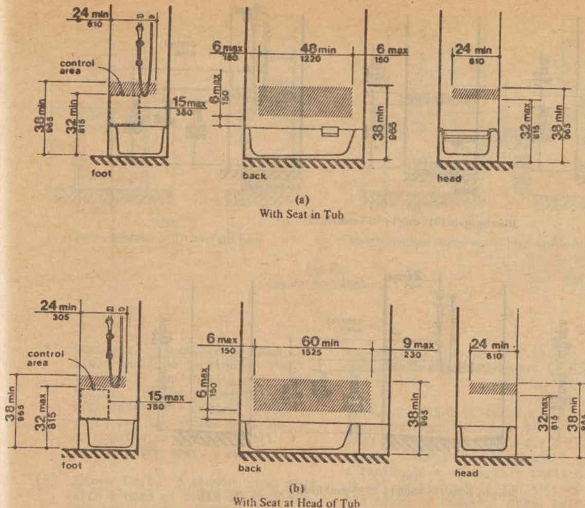
Fig. 48 Location of Grab Bars and Controls of Adaptable Bathtubs
