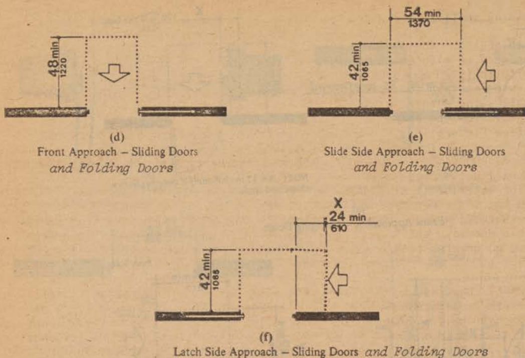
Fig. 25 Maneuvering Clearances at Doors (Continued)
