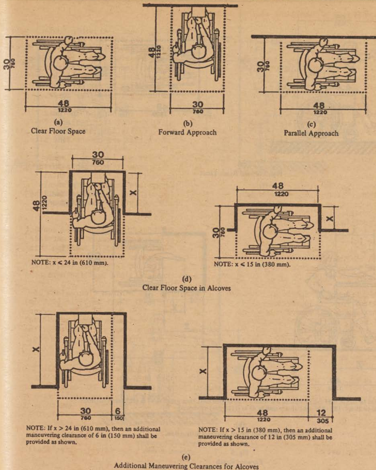
Fig. 4 Minimum Clear Floor Space for Wheelchairs
