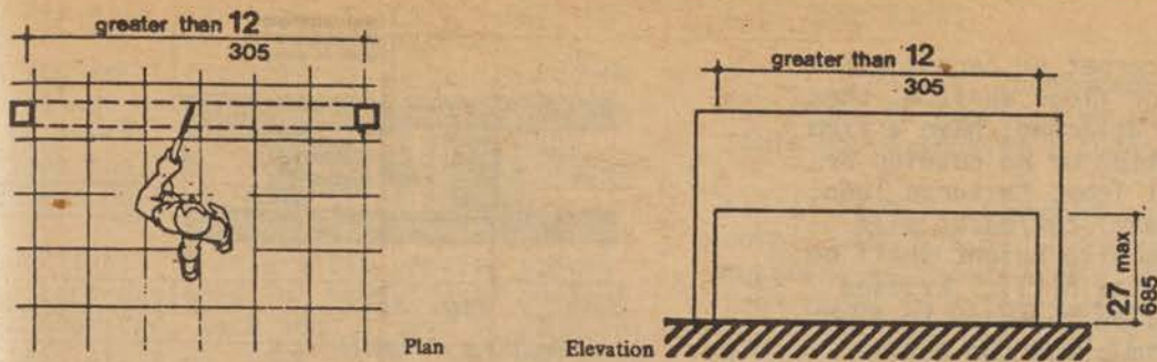
Free-Standing Overhanging Objects
