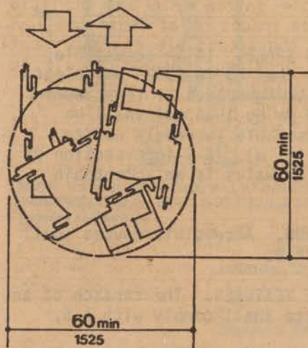
(a) 60-in (1525-mm) -Diameter Space
