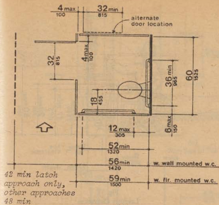
(a) Standard Stall
