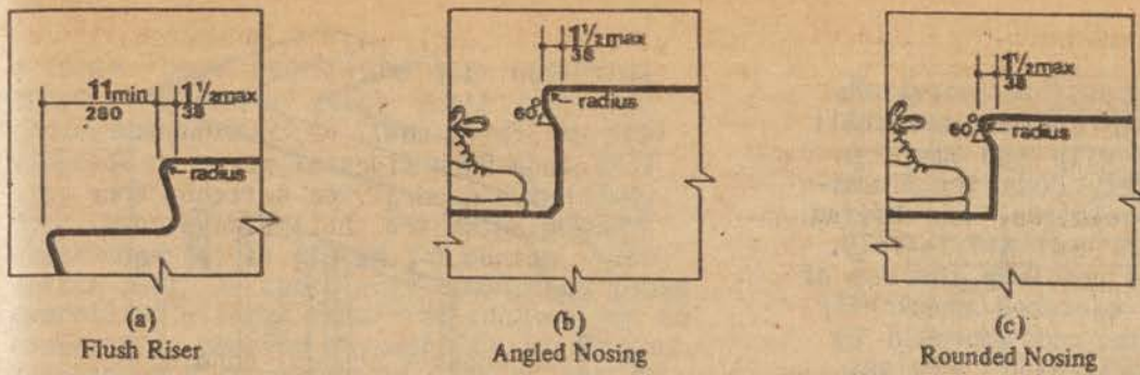
Fig. 18 Usable Tread Width and Examples of Acceptable Nosings
