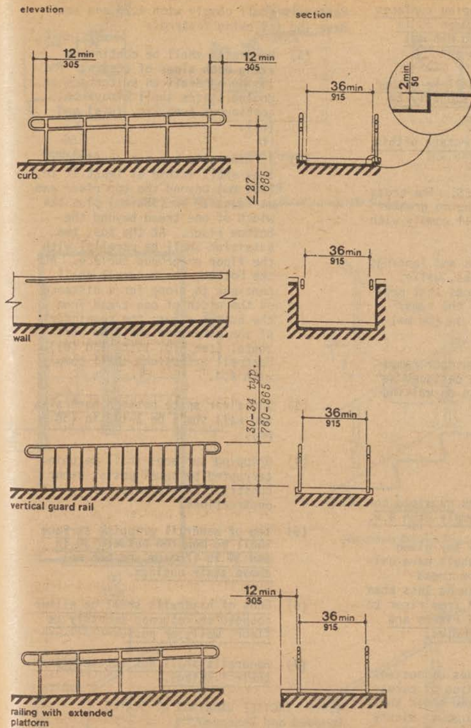
Fig. 17 Examples of Edge Protection and Handrail Extensions
