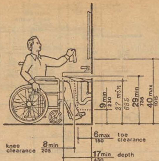
Fig. 31 Lavatory Clearances
