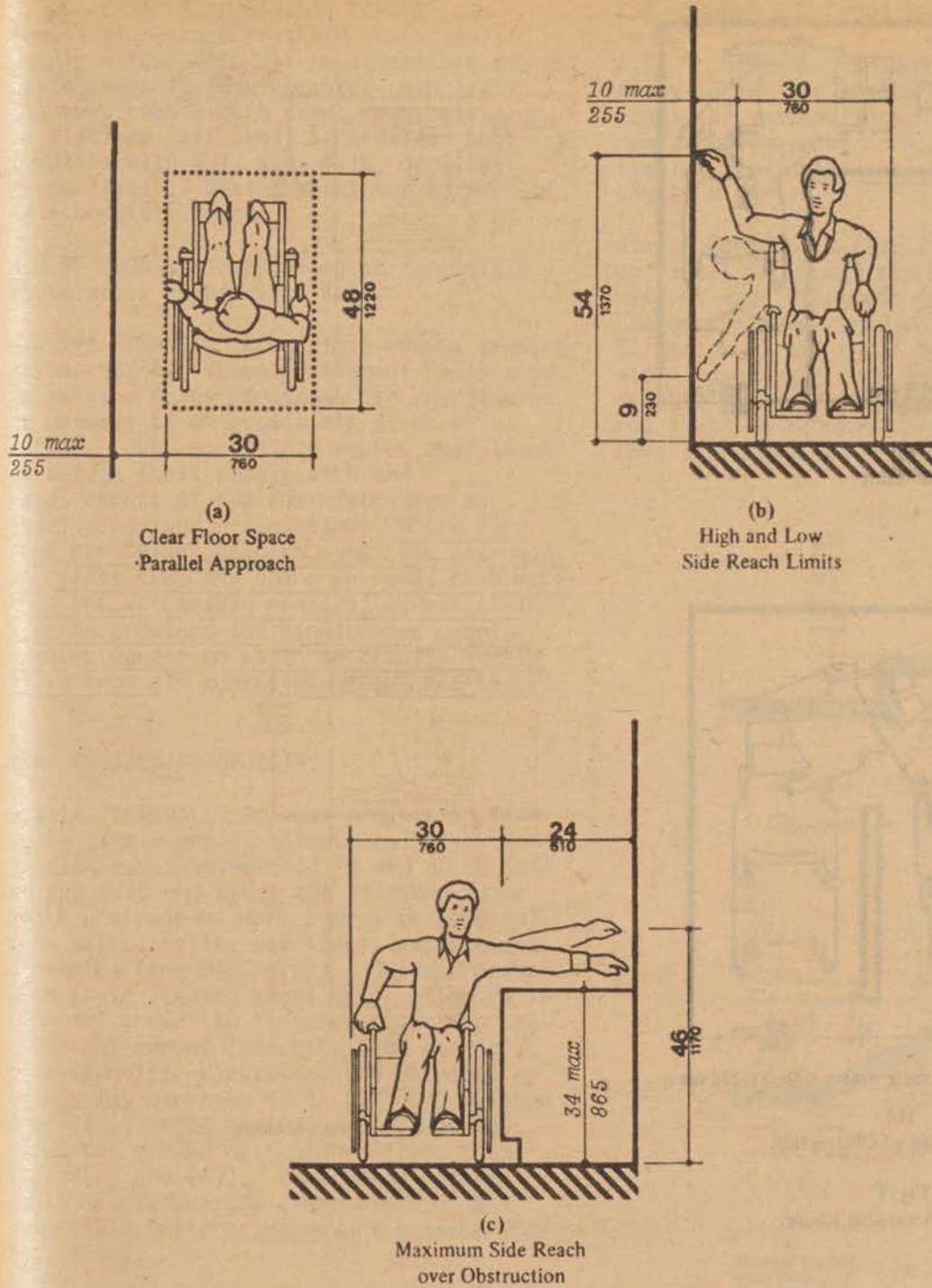
Fig. 6 Side Reach
