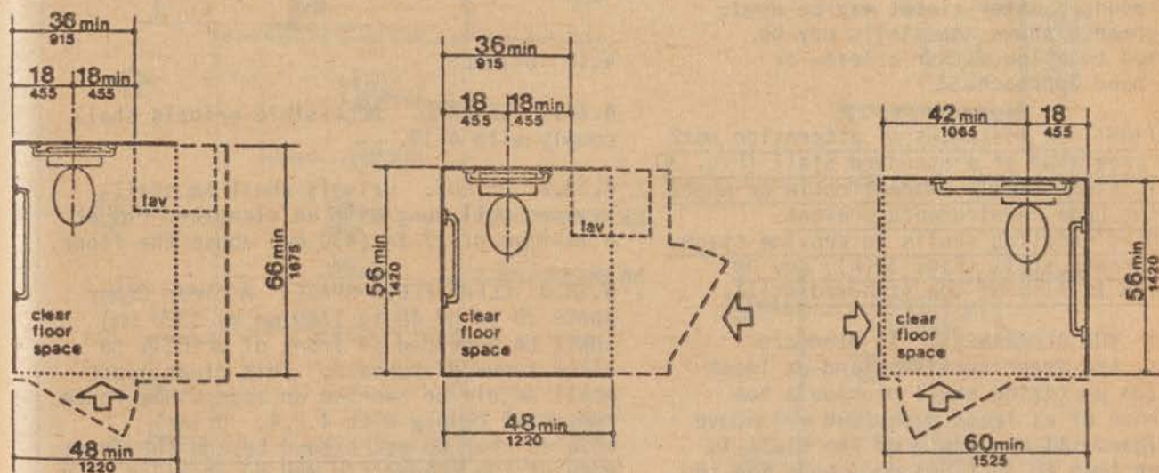
Fig. 28 Clear Floor Space at Water Closets
