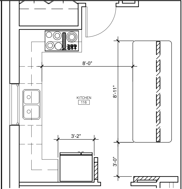
ENLARGED KITCHEN PLAN 1/4" = 1'-0" 02
