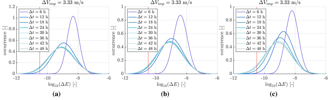
Figure 6: The plot displays the thrust energy normal distributions associated with every \Delta t covering a radial (a), transverse (b), and normal (c) 3.33 \text{ m/s} magnitude maneuver. As \Delta t between BCs increases, a shift towards lower magnitudes is noticeable as progressively cheaper maneuvers are found as optimal solutions. The vertical red line represents the impulsive maneuver thrust energy, acting as a lower bound.
