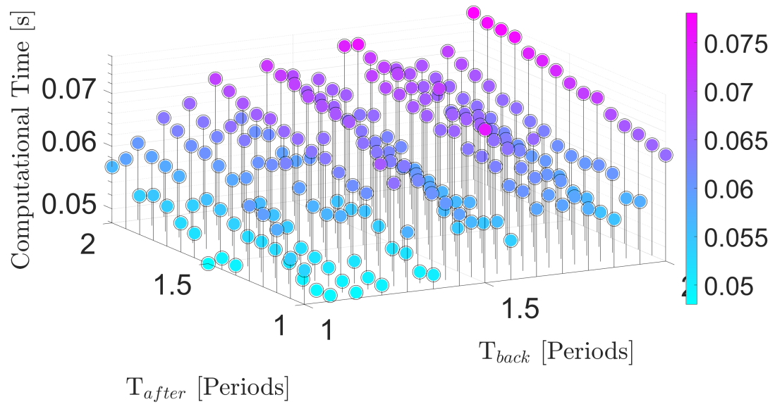
Figure 7: EO PTP computational time
