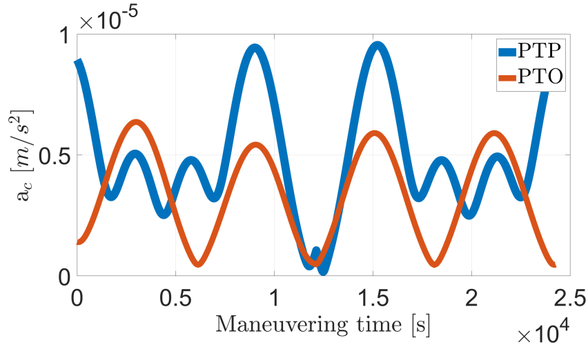
Figure 10: Acceleration magnitude comparison between PTP and PTO for T_{back} = 2 \text{ periods} and T_{after} = 2 \text{ periods}
