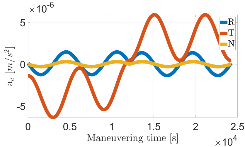
Figure 11: PTO Acceleration components in RTN for T_{back} = 2 \text{ periods} and T_{after} = 2 \text{ periods}
