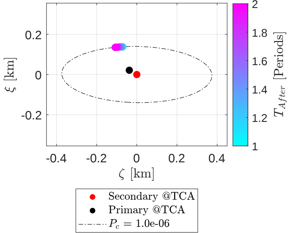
Figure 8: B-plane representation for the EOP PTO solution.
