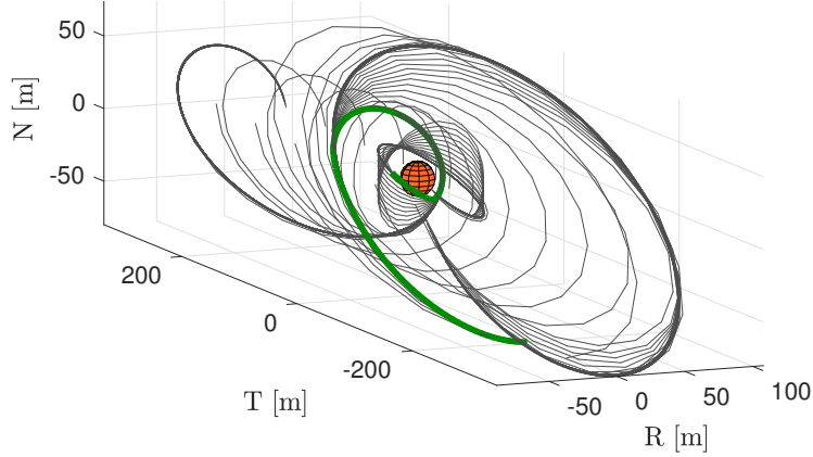
Figure 7: Uncontrolled relative trajectories propagated from each of the PAS nodes for 1 orbital period for the PAS-CAR case with M = 20 . The nominal trajectory is shown in green.
