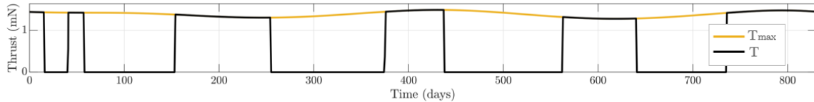
Figure 1. The typical bang-bang fuel-optimal thrusting profile.
