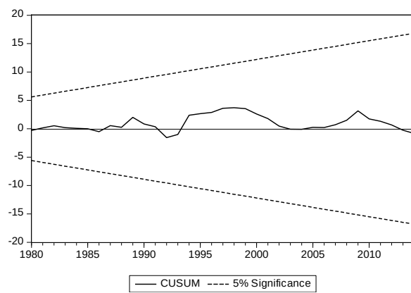
Figure 1. Cusum and Cusumsq tests
