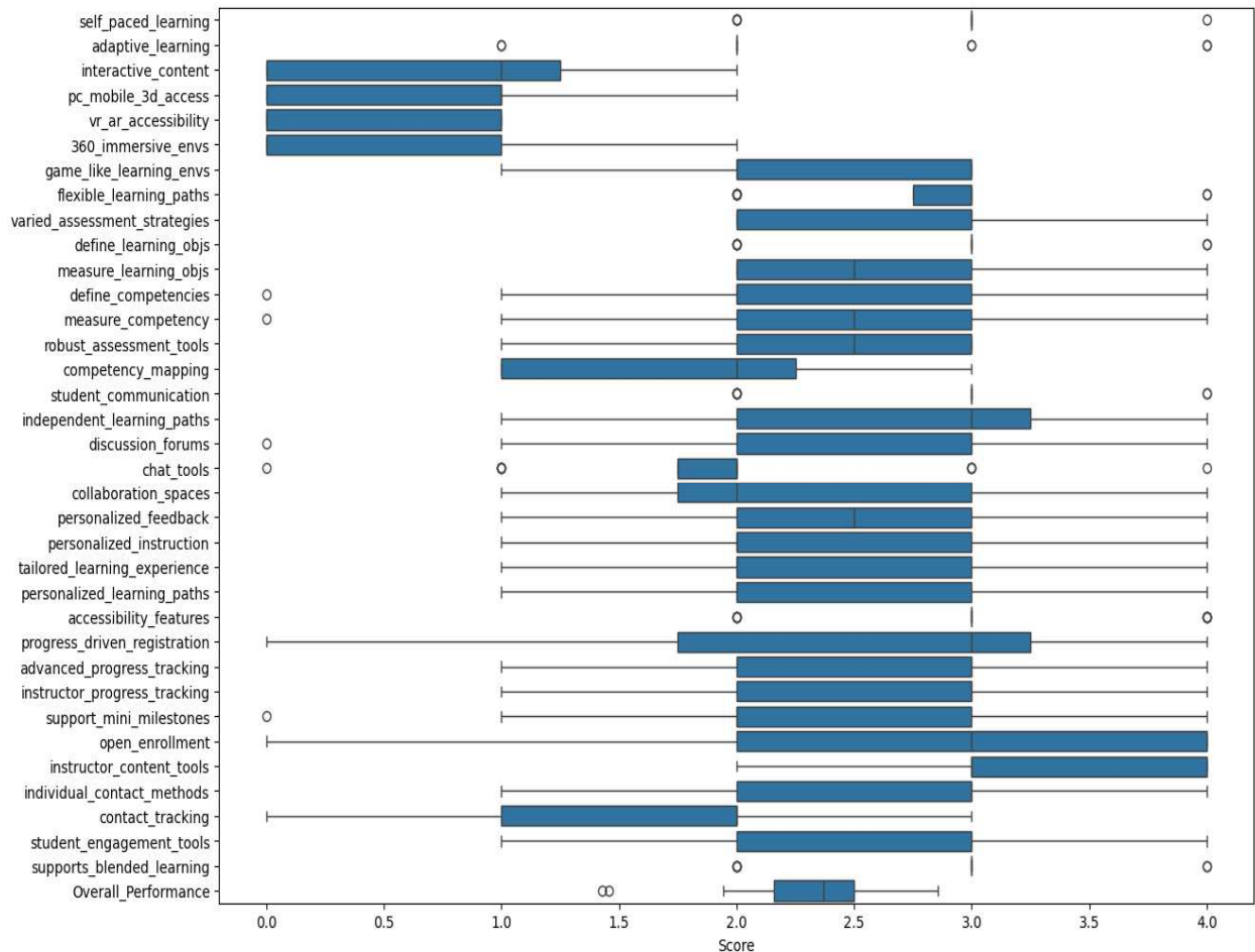
Figure 1 Distribution of Scores Across Different Criteria
