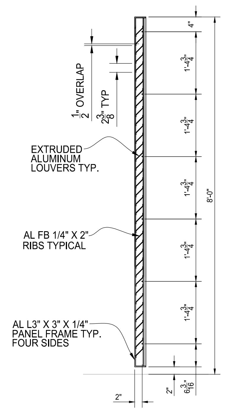
B TYPICAL PANEL SECTION
