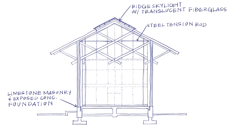
② BUILDING SECTION
