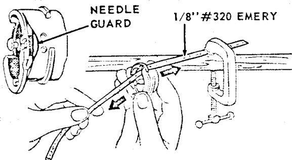
Fig. 54. Stringing Needle Guard
