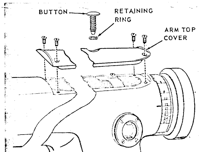
Fig. 33. Removing Stitch Length Regulator Button
