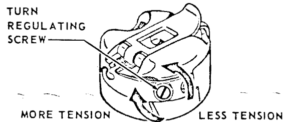
Fig. 25 Bobbin Thread Tension
