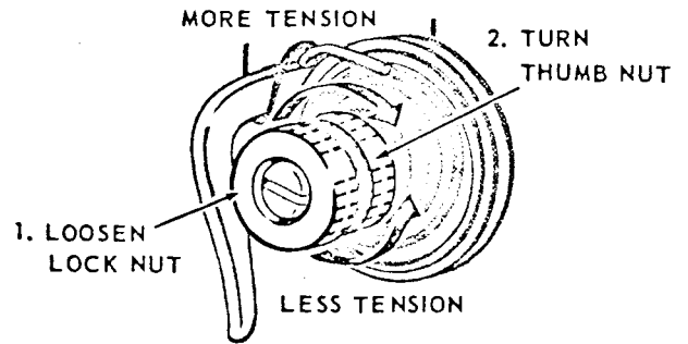
Fig. 24. Needle Thread Tension
