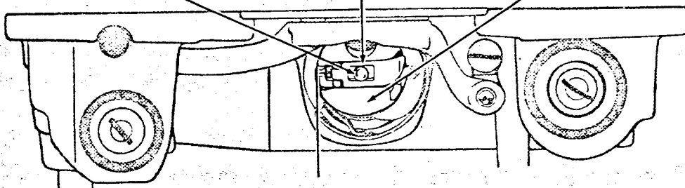
Fig. 23. Replacing Bobbin Case
