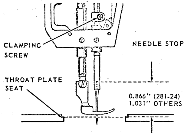
Fig. 41. Setting Needle Bar at Correct Height (Using Gauge Distance)
