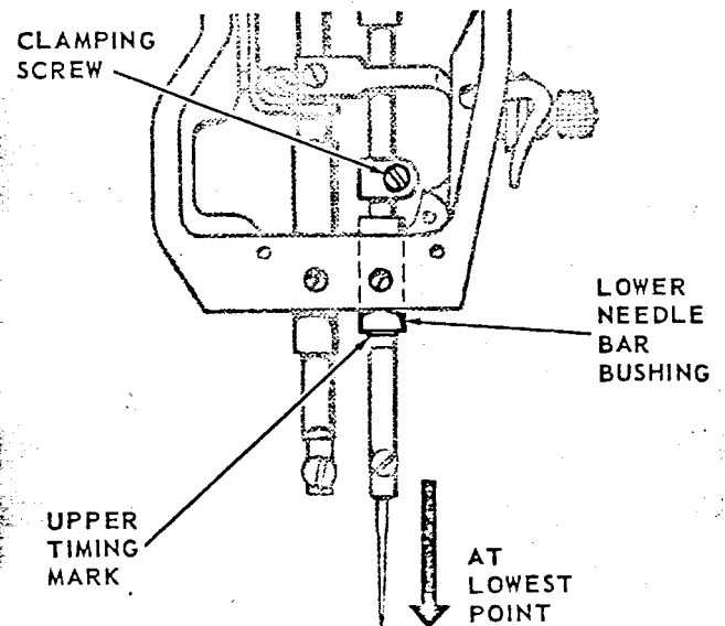
Fig. 43. Setting Needle Bar at Correct Height on all Machines, except 281-22 and 281-24
