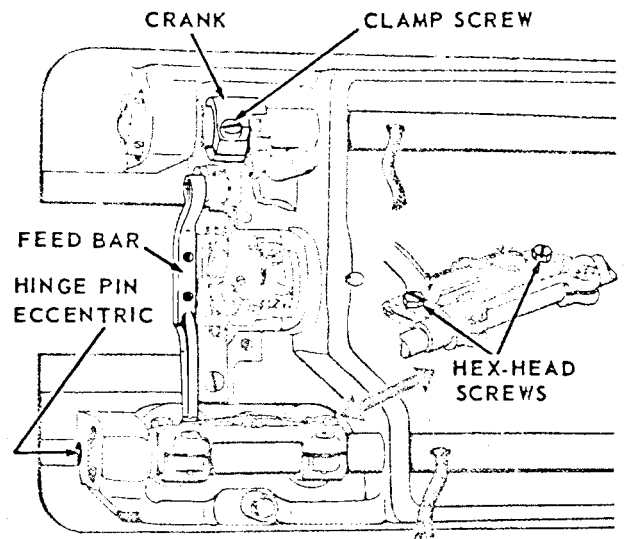
Fig. 60. Feed Bar and Crank
