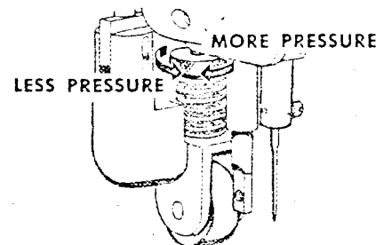
Fig. 27. Regulating Pressure of 281-20 281-30 Roller Presser on Machine 281-20
