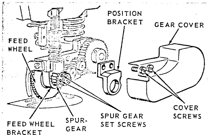
Fig. 64. Changing the Feed Wheel on Machine 281-23
