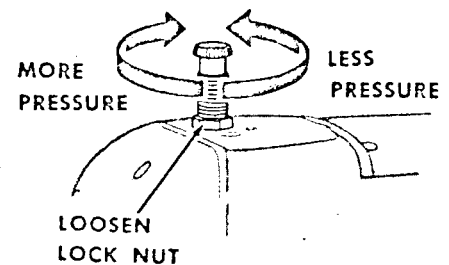
Fig. 26. Presser Foot Pressure
