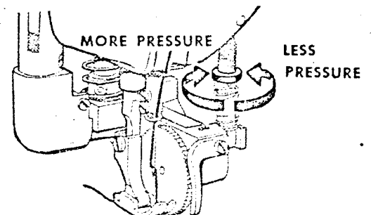
Fig. 28. Regulating Pressure of Roller Presser on Machine 281-23
