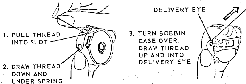
Fig. 22. Threading Bobbin Case
