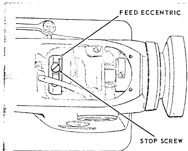
Fig. 61. Feed Eccentric Stop Screw
