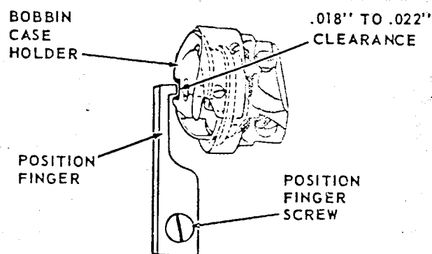
Fig. 50. Position Finger
