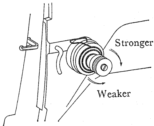
Fig. 20 Thread tension nut
