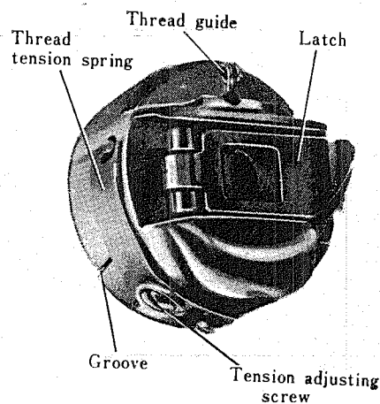
Fig. 13 Part names of the bobbin case
