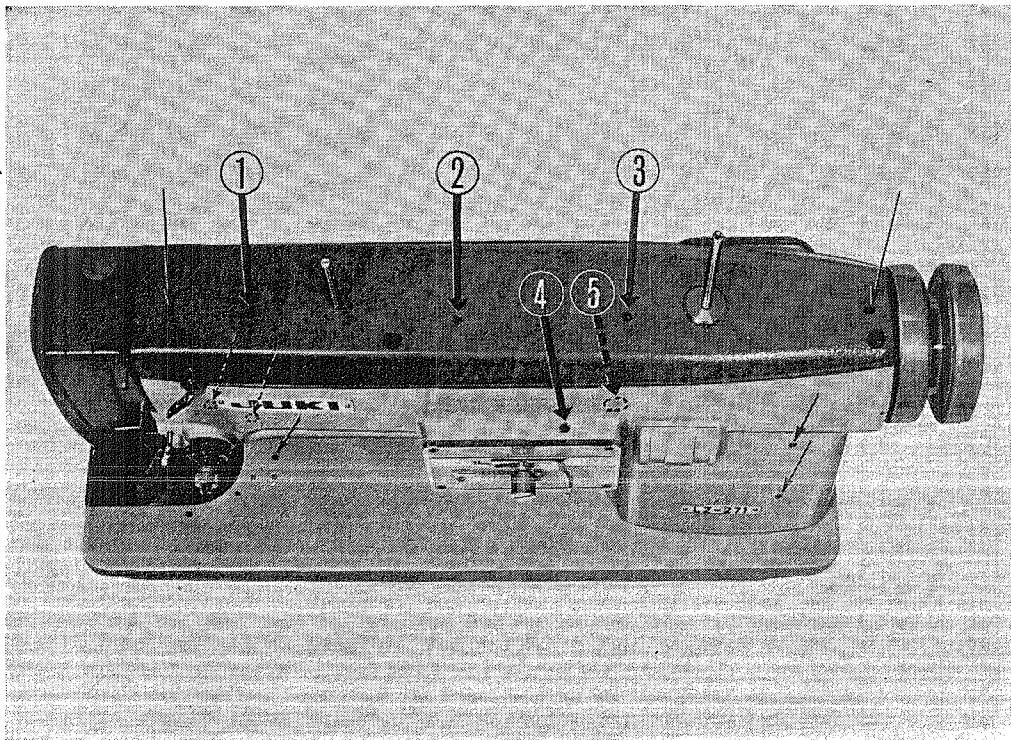
Fig. 5 Oiling holes
