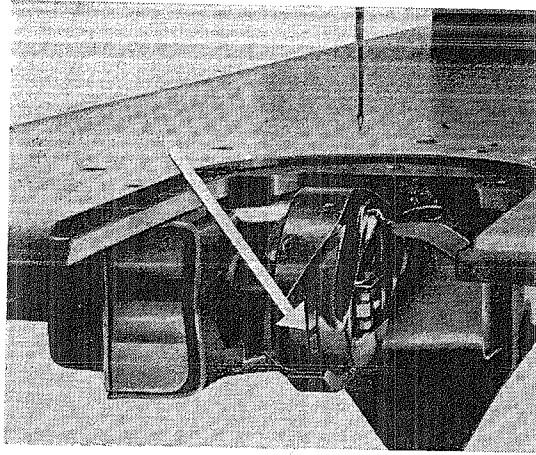
Fig. 6 Oiling spots of rotary hook
