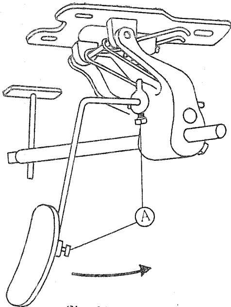
Fig. 14 Action of the knee press
