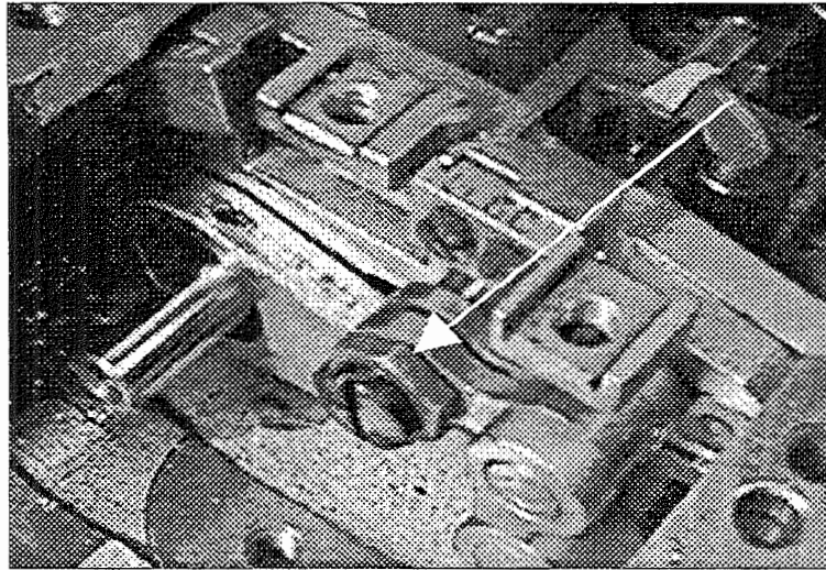
FIG 20. Install the eccentric bushing (34337F) with its screw through the drive link (34336A) and secure the screw to its hole in the feed bar assembly.
