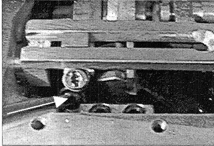
FIG 19. Continue pushing the thrust collar through its next bushing and into the differential feed lever.
