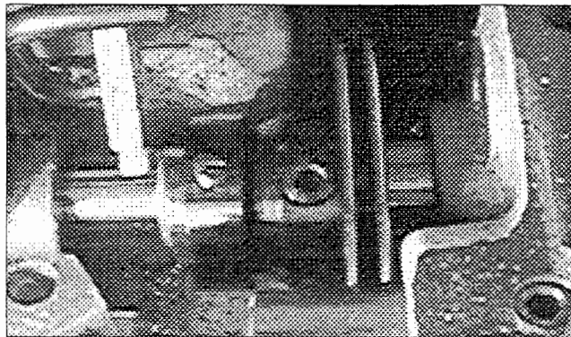
FIG 11. Push the stop collar (34366) to the right against the take up cam and secure its screw.
