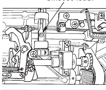
❶ Knee lifter lever shaft spring setscrew SM5030455SF
