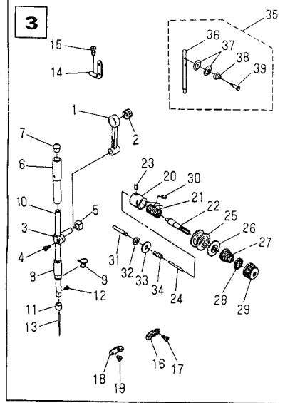
3. Needle bar & thread tension components
