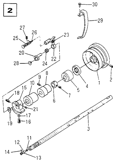
2. Main shaft & thread take-up components
