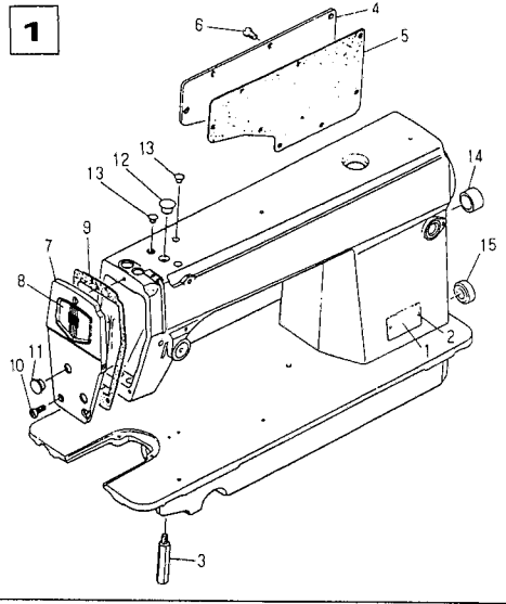
1. Arm bed components
