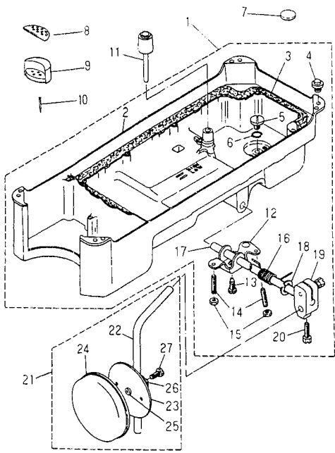
Oil reservoir &amp; knee lifter components
