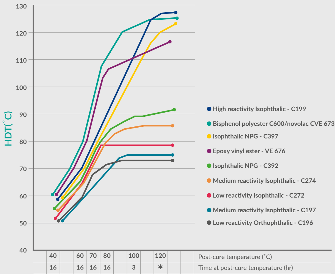
HDT level by post cure temperature
