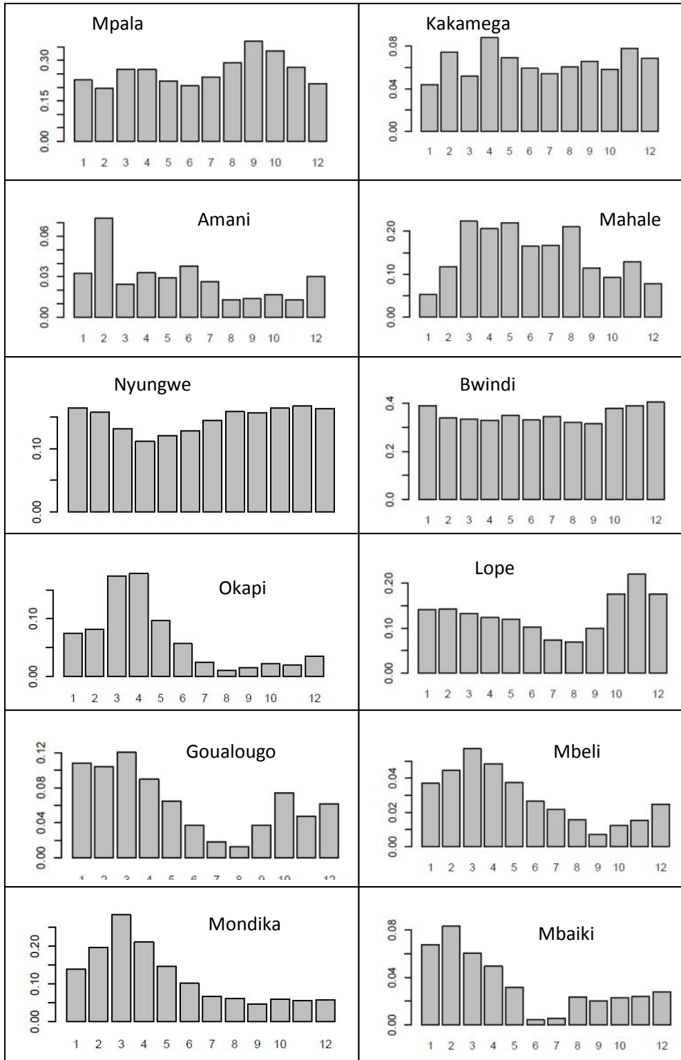
Figure 5. Seasonality in flowering at the sites plotting the proportion of trees flowering for each month of the year (1=January to 12=December).
