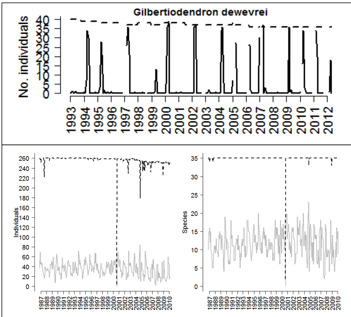
Figure 2. a) The number of Gilbertiodendron dewevrei trees flowering at the Okapi Faunal Reserve (top). b) The number of individuals flowering per month at Lope Reserve in Gabon (left) and number of species flowering per month (right). The black dotted lines at the top indicate the number of individuals/species being monitored in any month.
