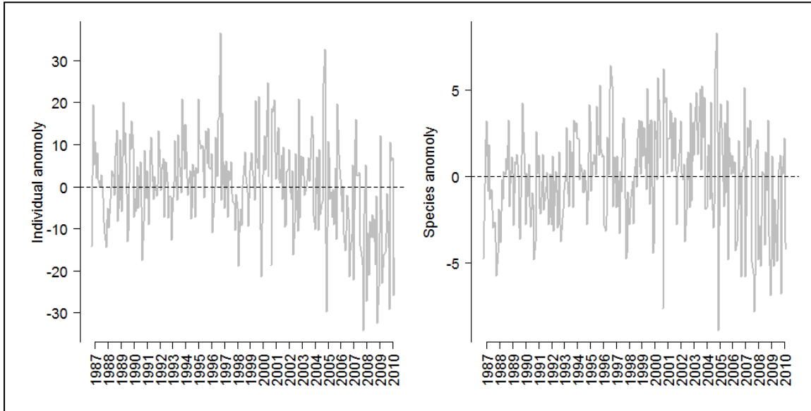
Figure 3. The anomaly between the value that month and the mean across the time period for flowering in the number of individuals (left) and the number of species (right) for Lope Reserve in Gabon. The anomaly indicates that there seems to have been a decrease in the number of individuals and species flowering since 2004.
