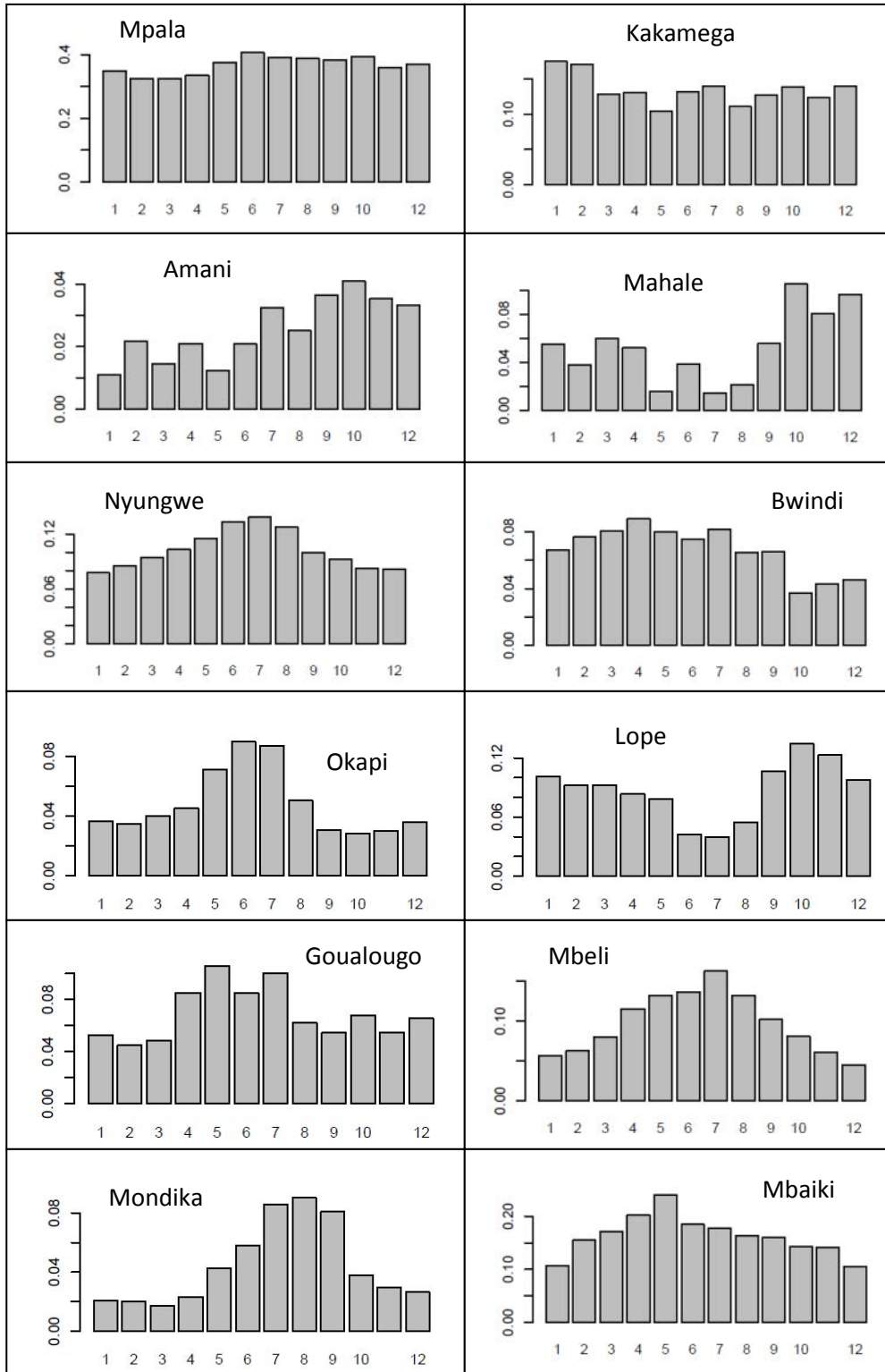
Figure 6. Seasonality in production of ripe fruit at the sites plotting the proportion of trees with ripe fruit for each month of the year (1=January to 12=December).
