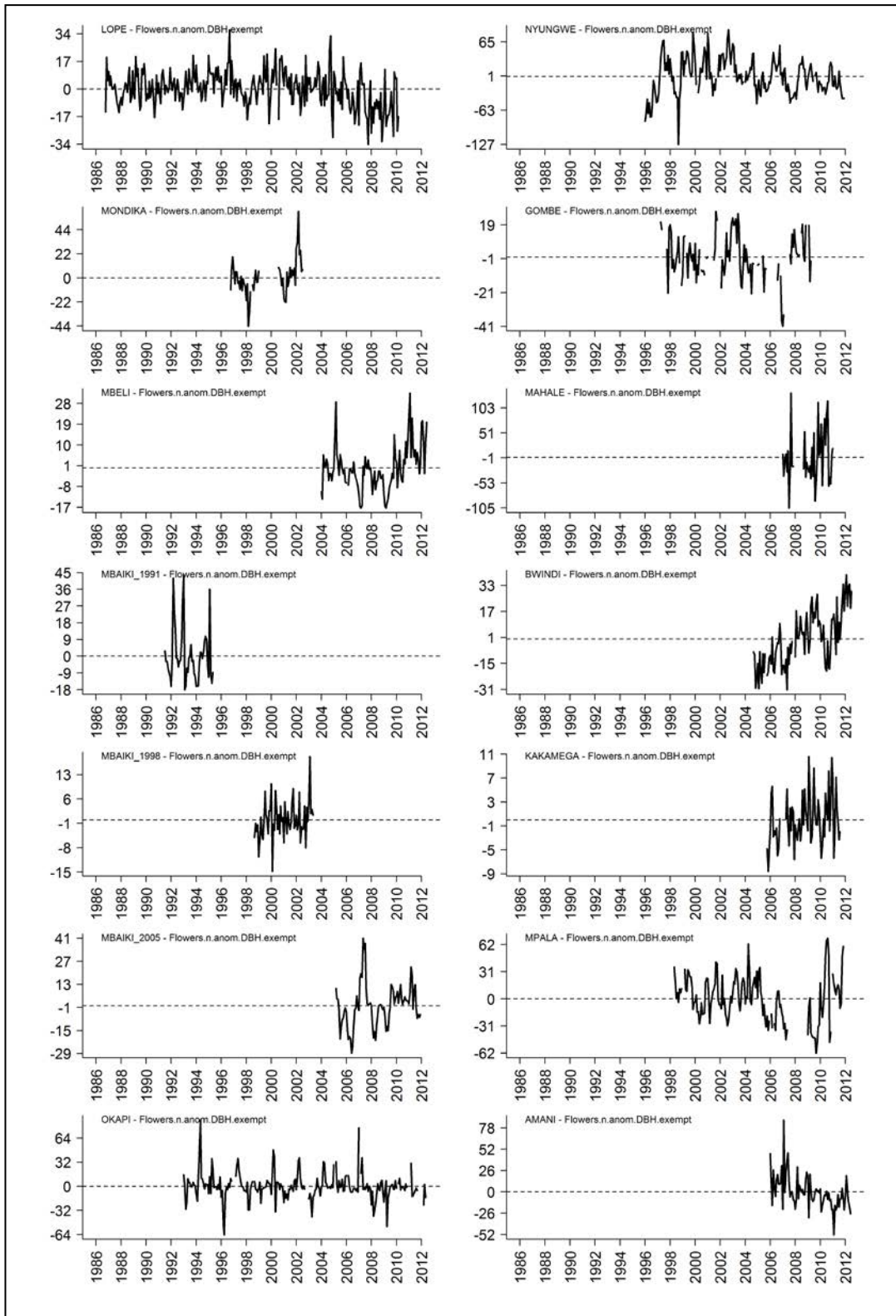
Figure 4. Comparison of the flowering anomalies of individual trees across 14 sites plotted on the same time line.
