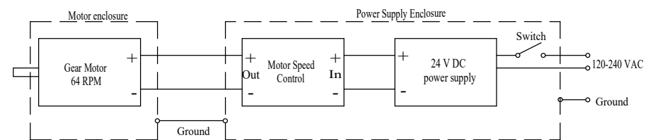
Star Roller Circuit Diagram
