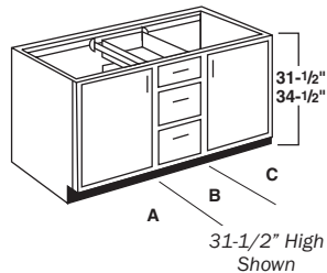
Cabinet face dimensions:
