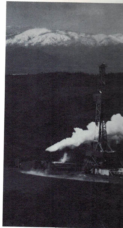
Geothermal well overlooking Clear Lake, California
