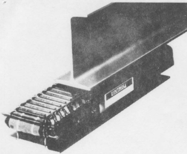
Fig. 5 The LIM: stator windings are mounted on top of the vehicle. The "rotor" is the guideway flange
