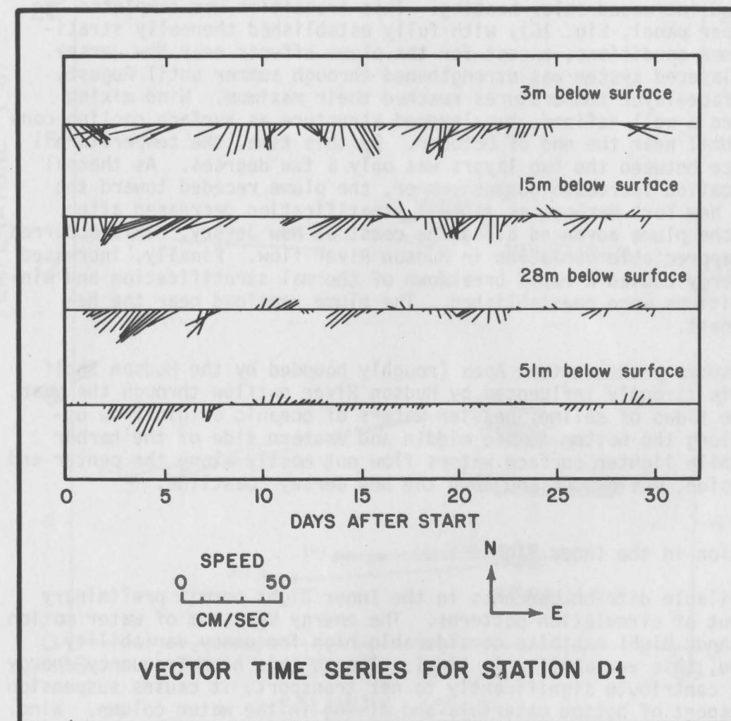
Figure 14. Variations of currents at Station D1 located within alternative dump site area 1-A. The bottom current meter, at a depth of 51 m, was 4 m above the sea floor.
