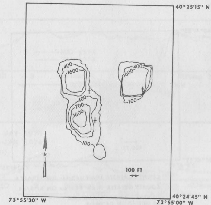
Figure 6. Dispersal pattern of gold-labeled tracer sand at end of Nov. 1973 experiment. Crosses show ship position at time of drop. See figure 5 for supplementary location information.
