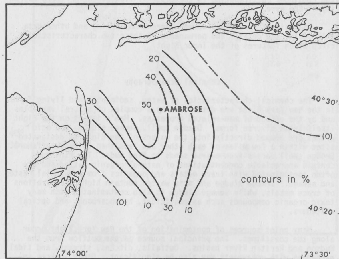
Figure 17. Percentage of seabed drifters recovered from the Hudson River estuary as a function of their initial location.
