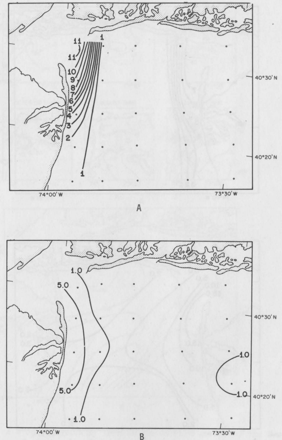
Figure 28. A - surface silicate, 16-20 September 1973. B - surface silicate, 25-29 November 1973 ( \mu\text{g} - atoms per liter).
