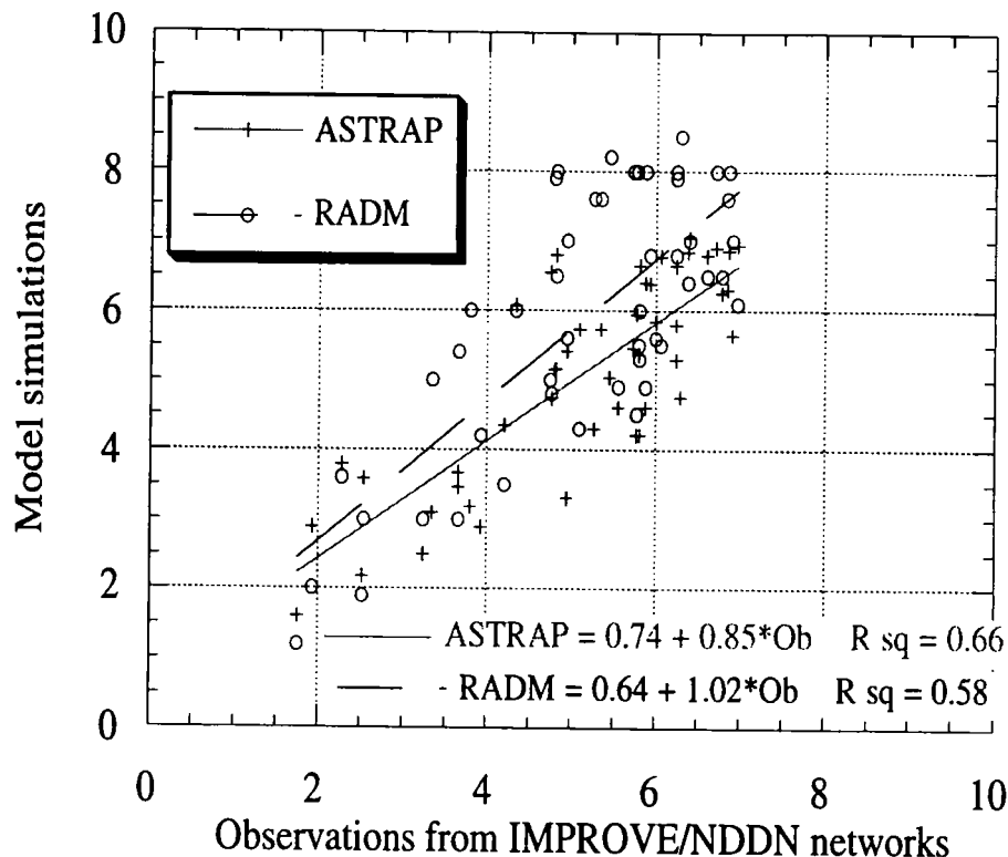
Figure 5: A comparison of predictions by ASTRAP (the TAF module) and RADM (another more detailed transport model) with actual observations of annual average concentrations of atmospheric sulfate ( \mu\text{g}/\text{m}^3 ) in the eastern United States in 1990.
