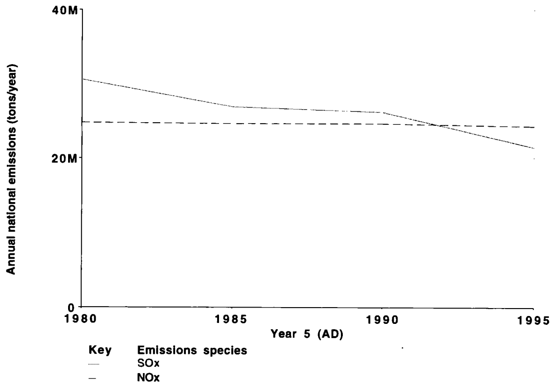
Figure 6. National SO x and NO x emissions.
