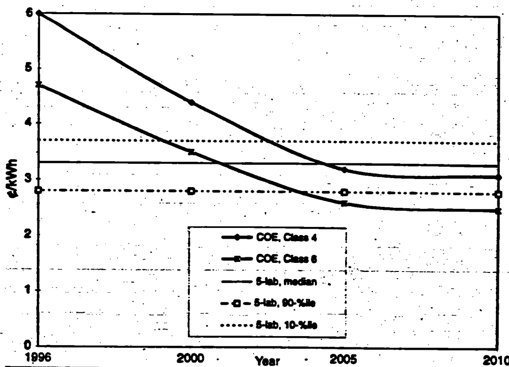
Figure 7.13 Projections of Wind Power Costs
