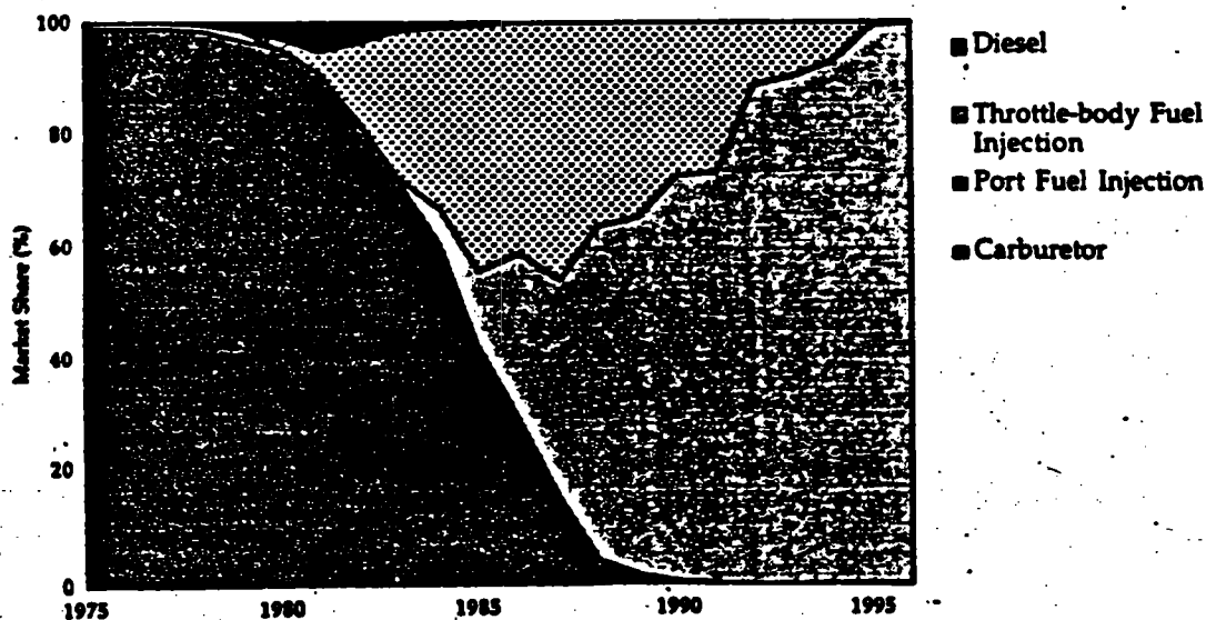
Figure 5.11 Penetration of Fuel Injection Technology
