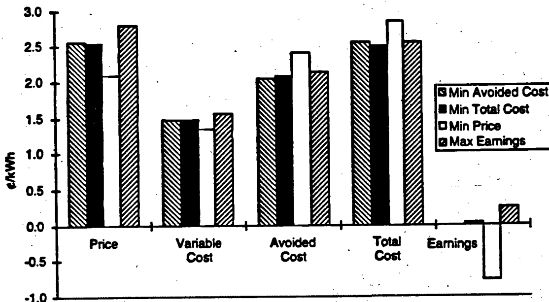
Figure 6.2 Generation Price and Costs using Different Optimizations (10% Fixed Reserve Margin)
