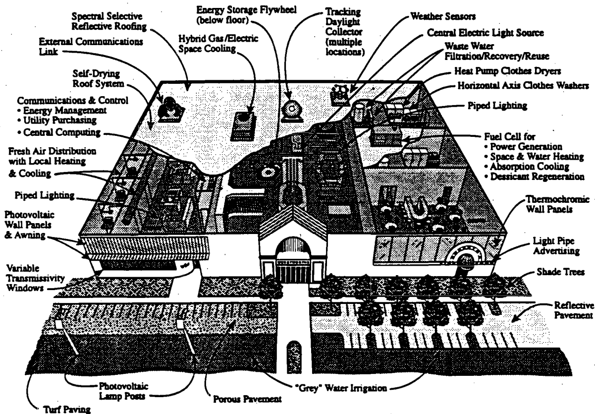
Figure 3.8 "Best Practice" Composite Commercial Building of the Year 2020
