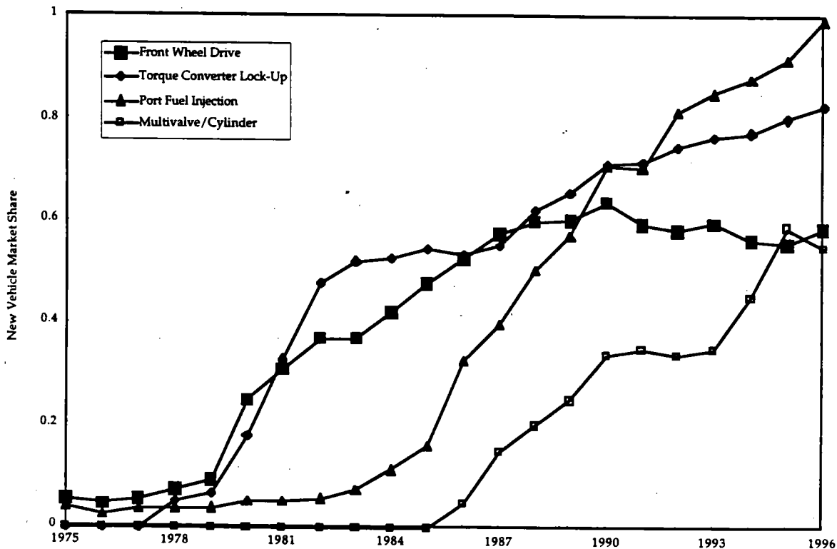
Figure 5.5 Use of Fuel Economy Technology In New Light-Duty Vehicles
