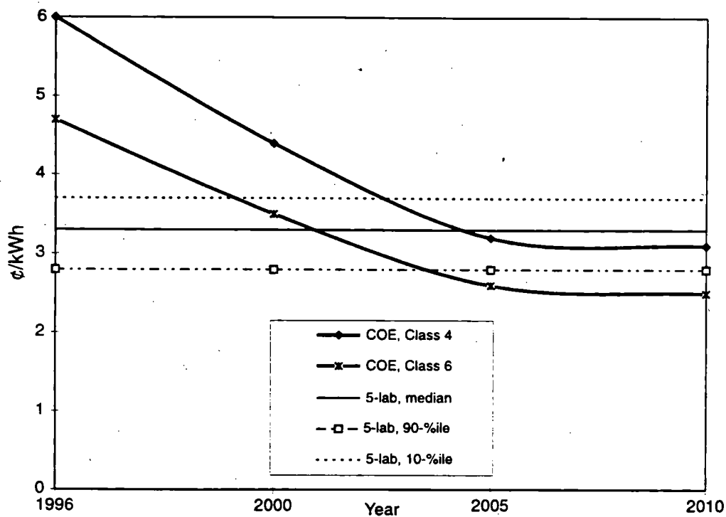
Figure 7.13 Projections of Wind Power Costs
