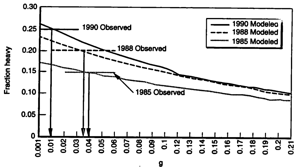
Figure 6.7—Fraction of Users That Are Heavy Users for Fixed a = 0.15 , b = 0.024 , and f = 0.04
