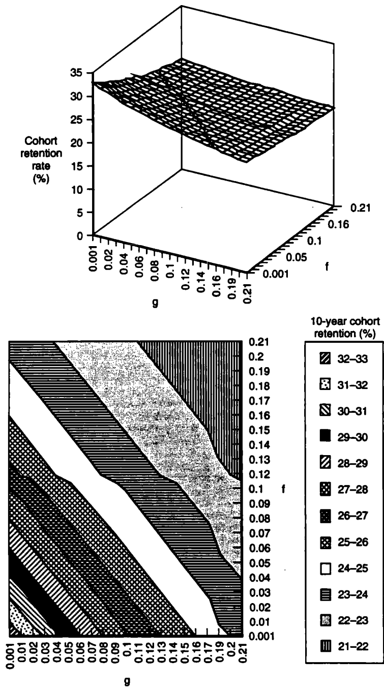
Figure 6.5—Ten-Year Cohort Retention for Fixed a = 0.15 and b = 0.024
