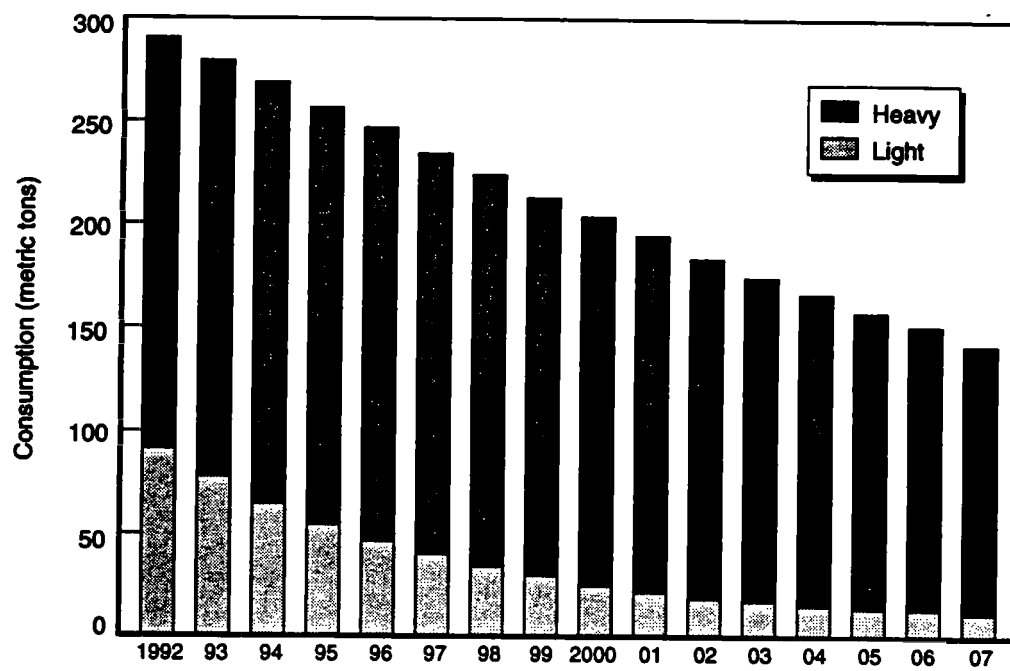
Figure S.11—Consumption Assuming Zero Incidence
