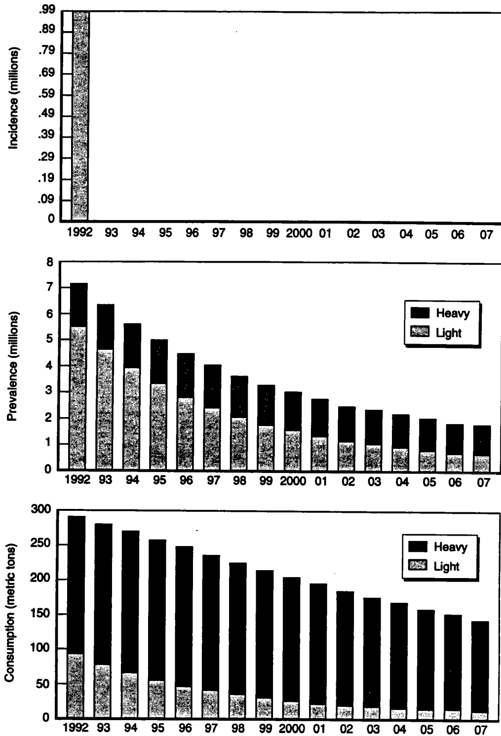
Figure 8.5—Hypothetical Scenario 5: Zero Incidence
