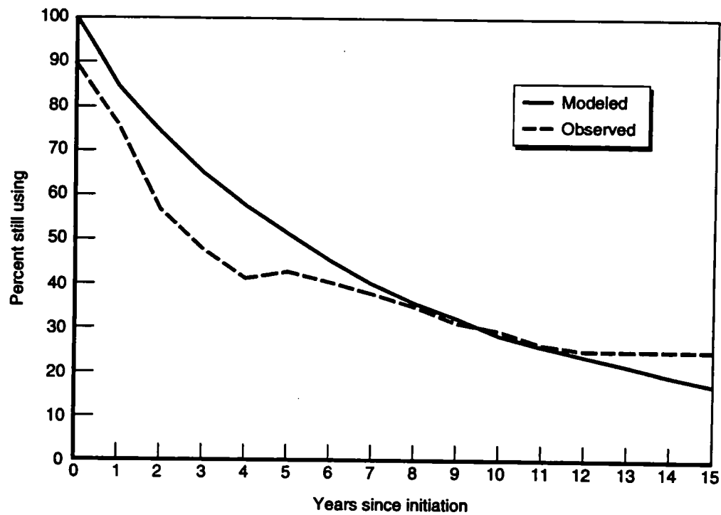
Figure S.4—Cohort Retention: Modeled vs. Observed
