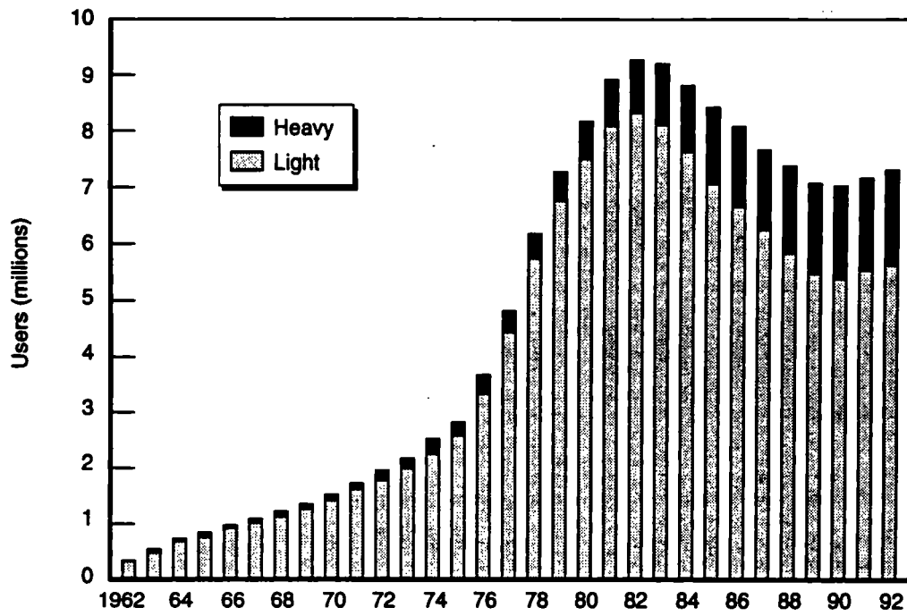
Figure 7.2—Modeled Prevalence: Heavy vs. Light Users
