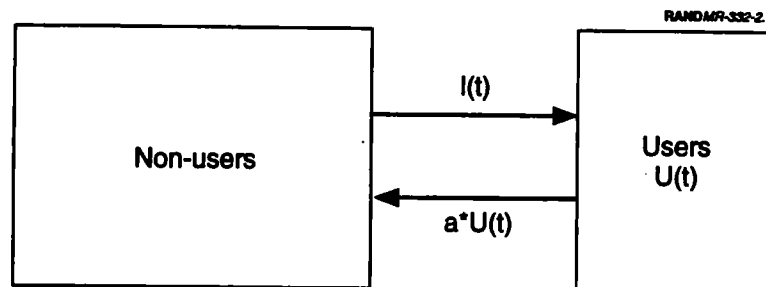
Figure 2.1—A One-State Markovian Model
