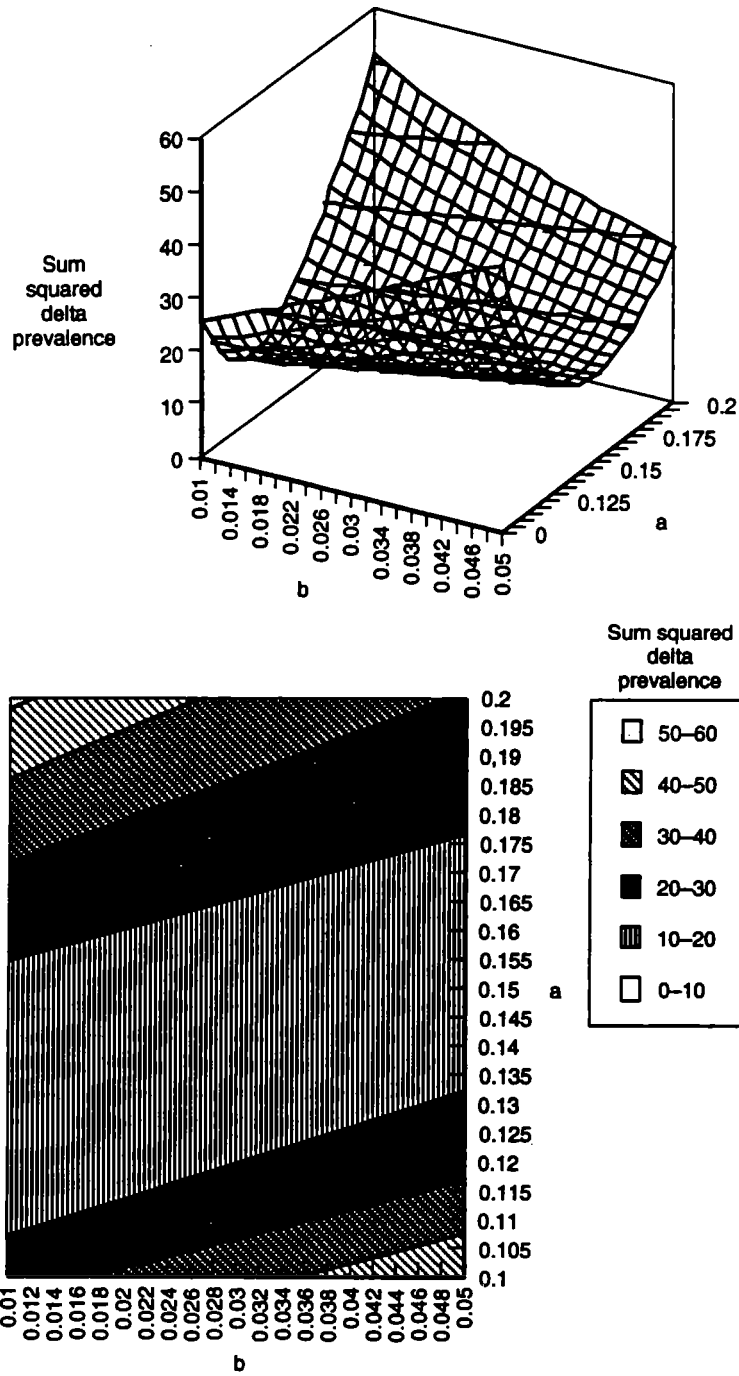
Figure 6.1—Sum Squared Delta Prevalence for Fixed f=0.04 and g=0.02
