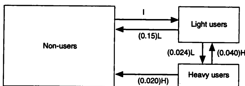
Figure 6.8—The Fitted Model
