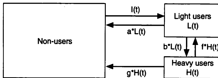
Figure 2.2—A Two-State Markovian Model
