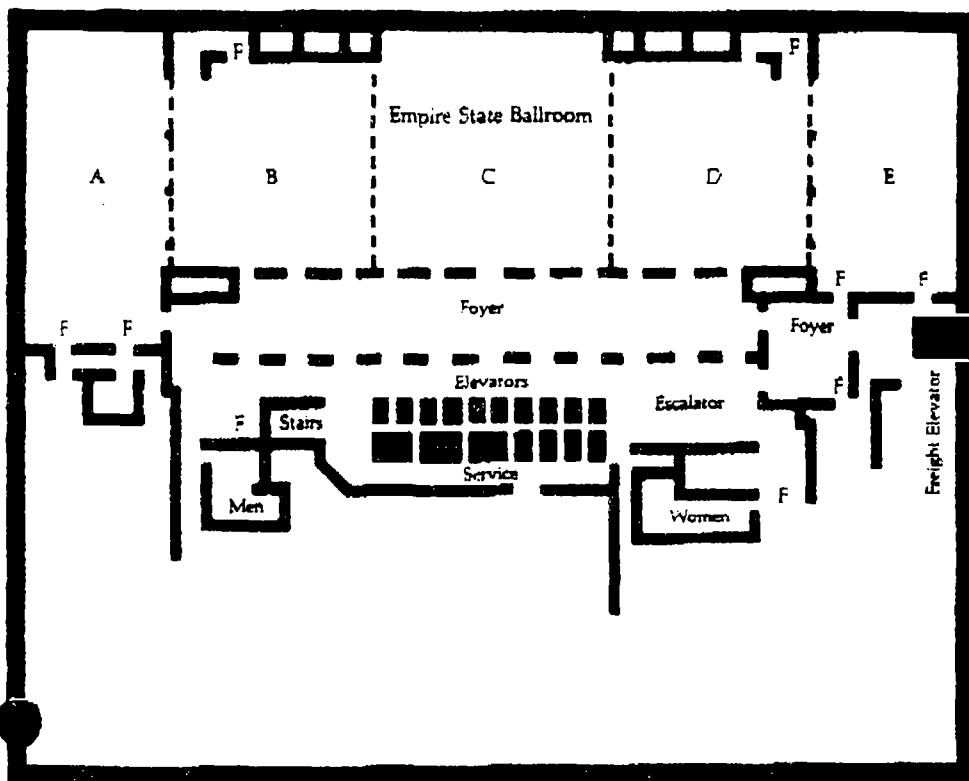
Ballroom Level
