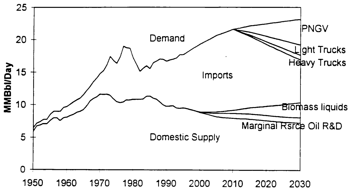
Figure ES-1. Potential Reduction of U.S. Oil Imports by Selected Advanced Technologies.
