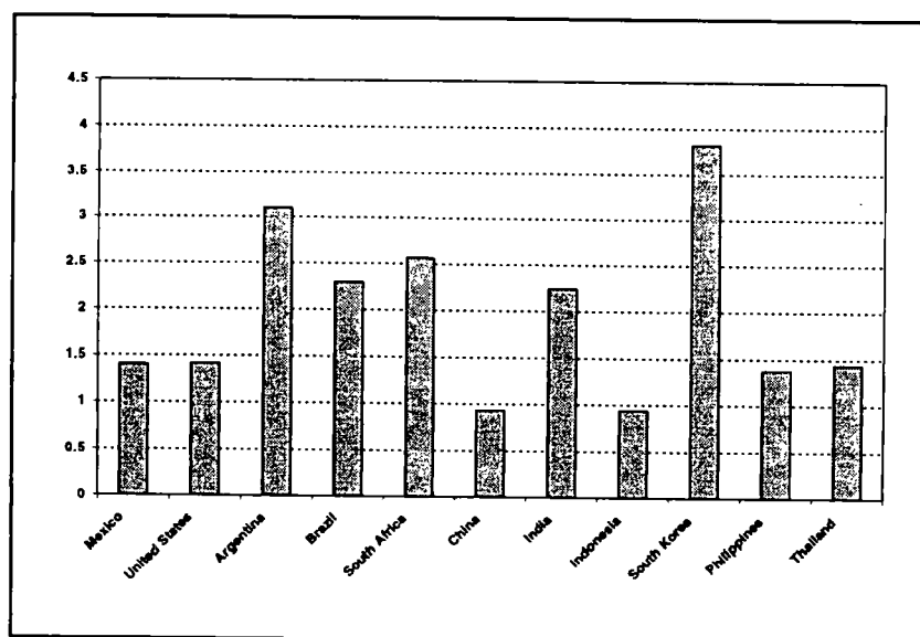
Exhibit 2-5 1998 Prices of Premium Unleaded Gasoline in Selected Countries Including Taxes
