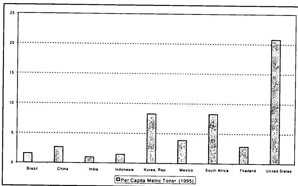
Exhibit 1-4: Metric Tons of Carbon per Capita for Selected Countries
