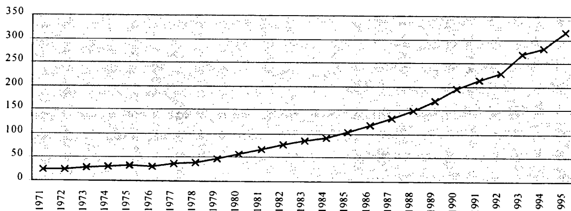
Exhibit D-7 KWh per Capita
