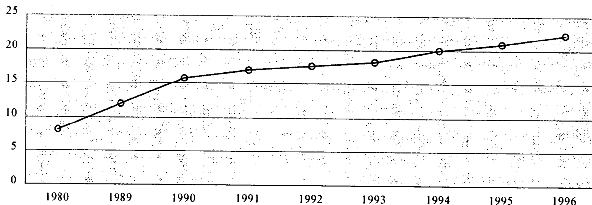
Exhibit D-6 Vehicles (per 1,000 people)
