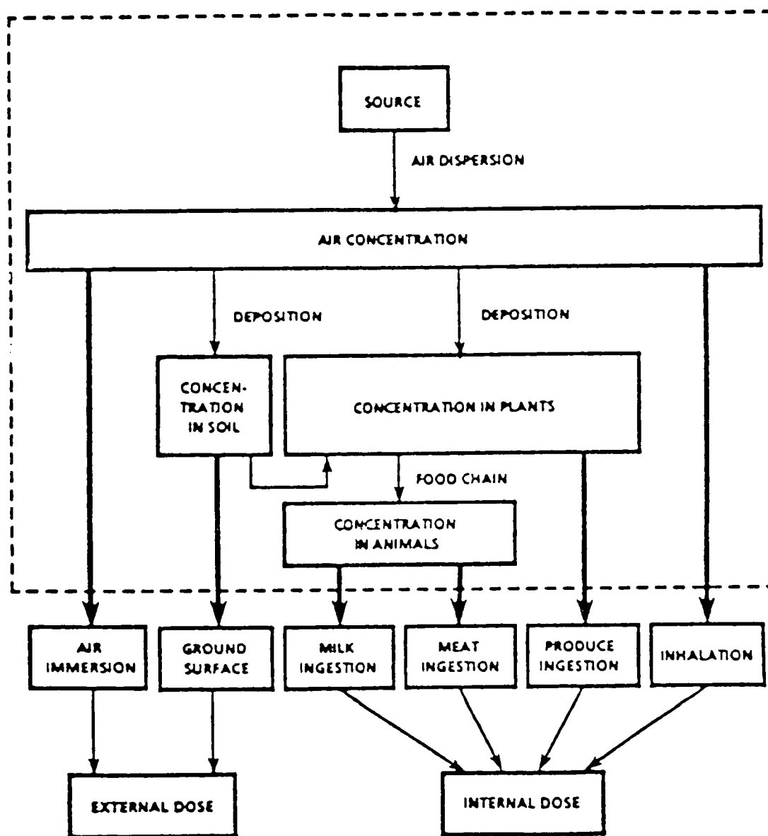
Figure 4-1. Pathways of airborne radionuclides into the environment.
