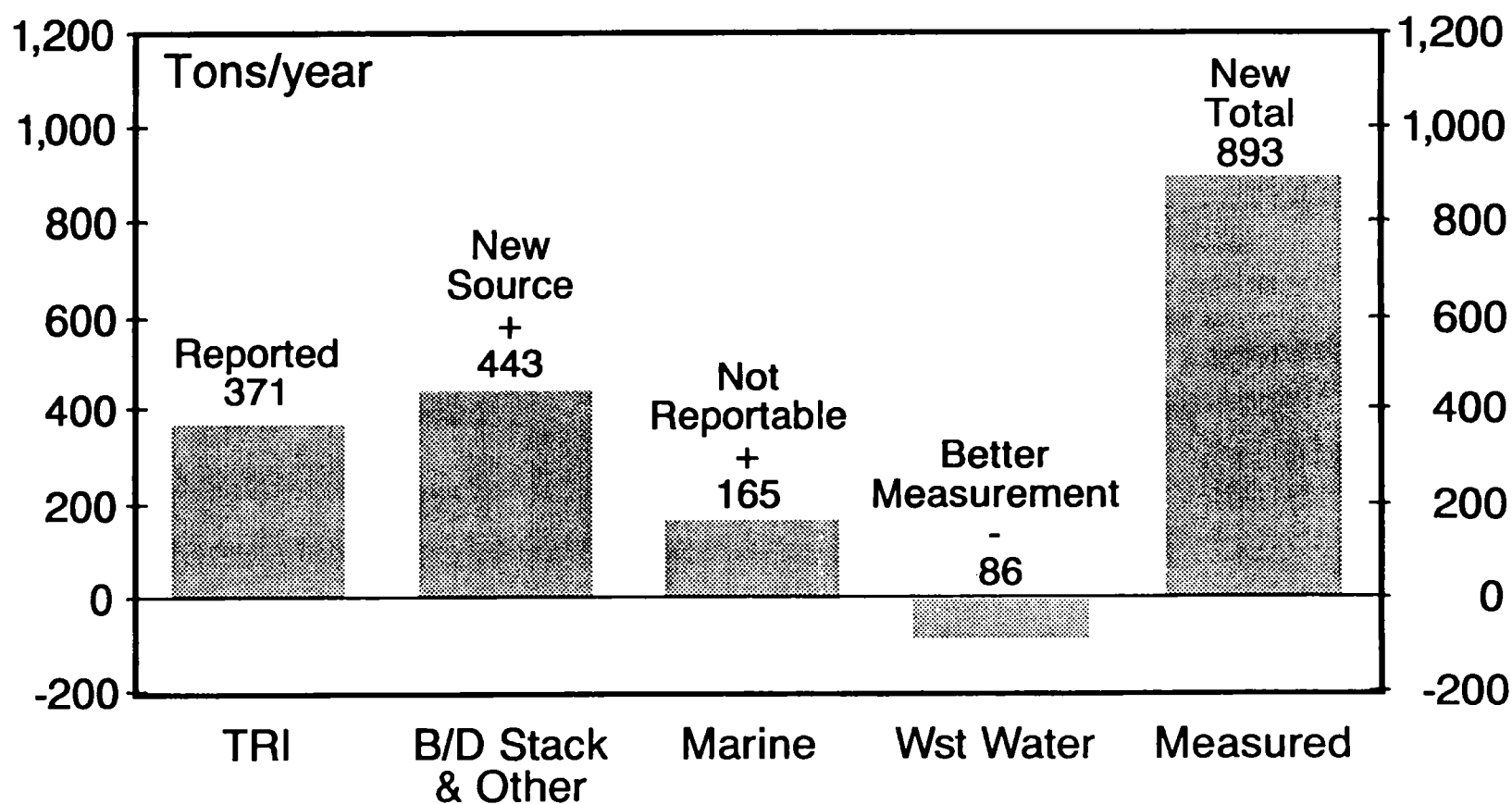
Figure 2.7 1989 TRI Inventory Compared to Measured Emissions
