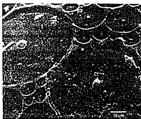
Colorized scanning electron microscope images of the surfaces of synthetic aluminophosphate spheroids reveal a pattern of micrometer bowls (left) and of "meshed" bowls that resemble the silica microskeletons of radiolarian, a single-cell organism (right). The two patterns are produced using slightly different chemical systems.
