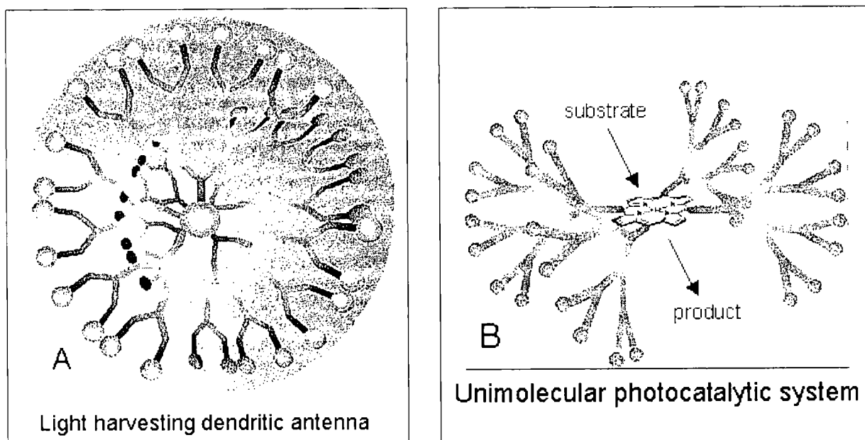
Figure 1. (A) Nanoscale light harvesting antenna based on a dendrimer. (B) Dendritic photocatalyst combining antenna and catalytic function.
