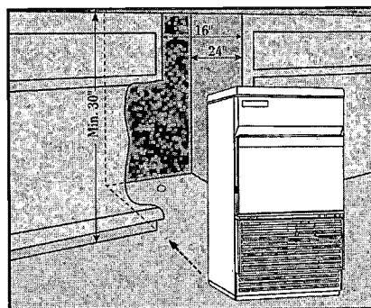
Cut-out dimensions for Model 3IMA
