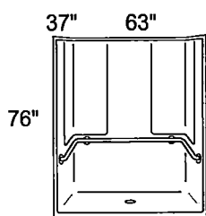
with wrap-around grab bar S-6337ADA2-C
