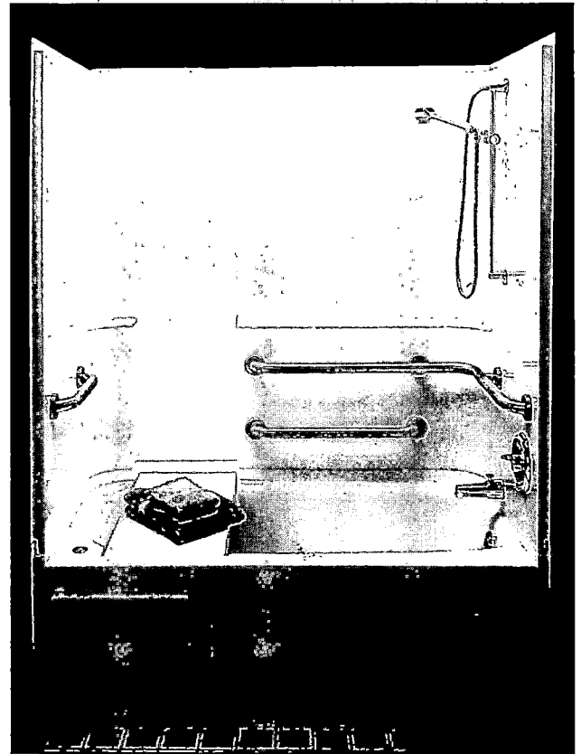
45R/LF Multi-piece right hand shown 60" x 36" x 79"
