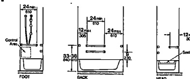
Figure 34(a)-ADA Section 4.20.4 Grab Bars
