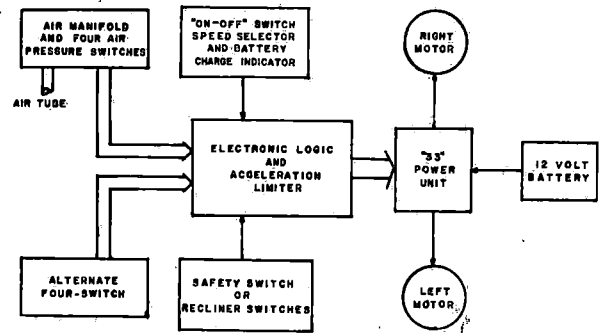
Figure 3. Diagram of controller
