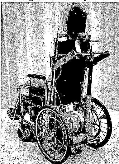
Figure 6. Photograph of recliner unit
