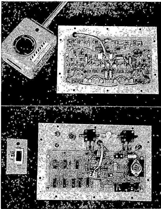
Figure 2. (A) Manipulandum and standard electronic control circuit for "33" chair, (B) Control box and replacement controller
