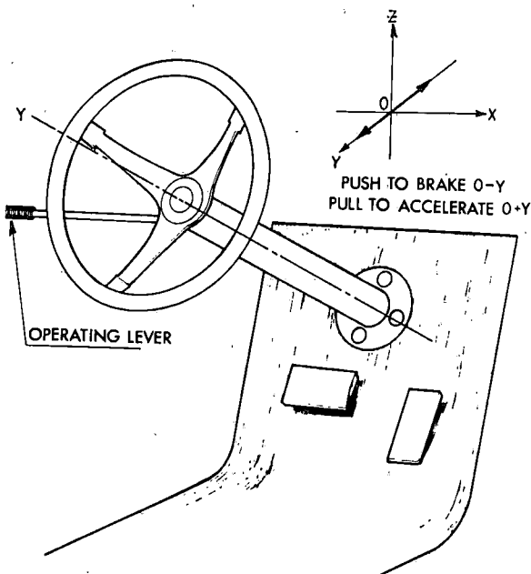
Fig. 1 Push-pull type control system
