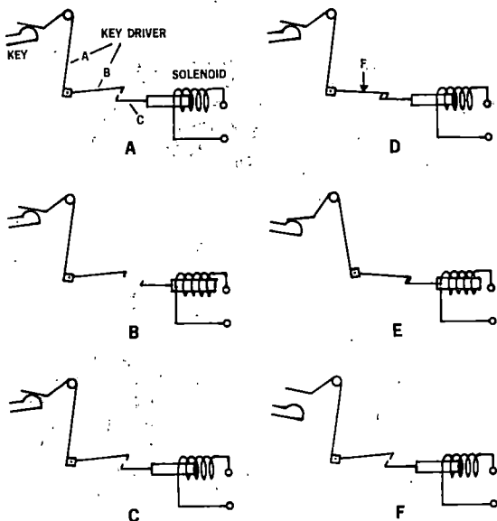
Figure 2. The operation of the key driver.
