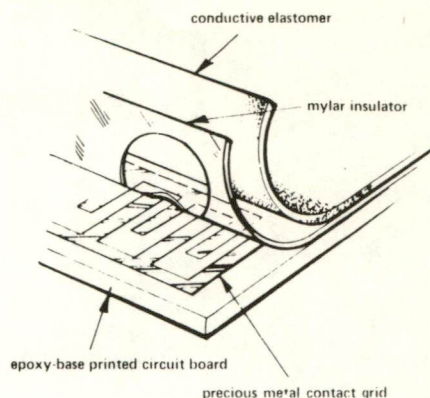
Elastomeric Switch Structure Fig. 4
