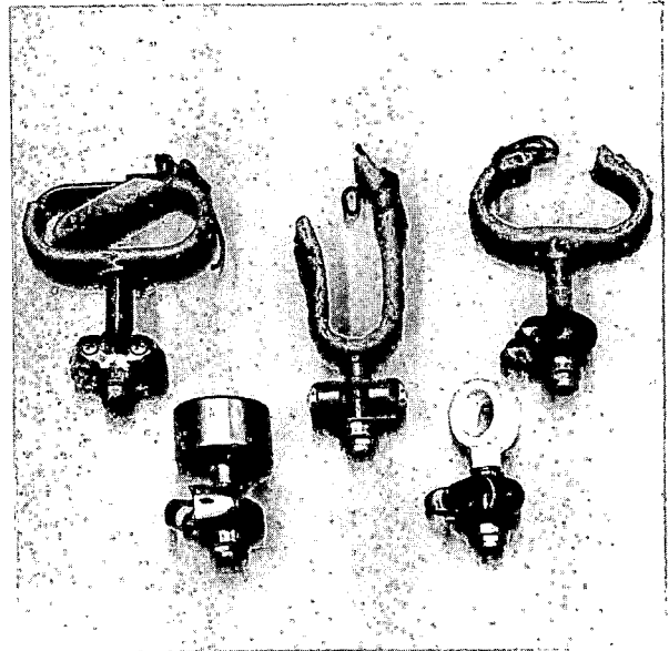
Fig. 4 Assortment of steering assists
