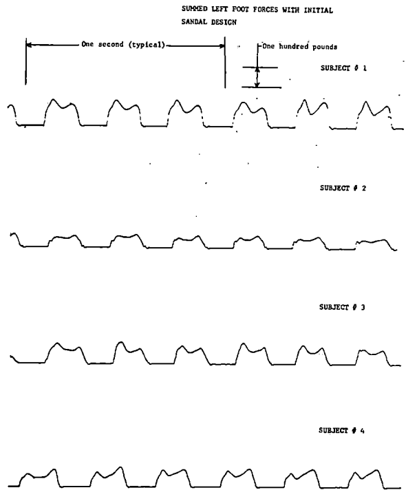
Figure 8 Typical Total Foot Force Variation During Walking of Various Subjects
