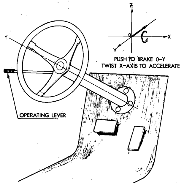
Fig. 3 Push-twist type control system
