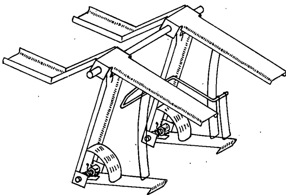
Figure 5. Detail of the record control key mechanism.
