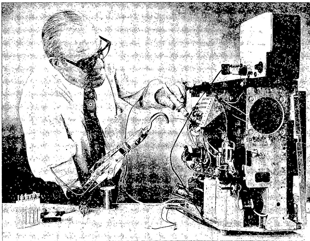
Fig. 1. Precision work can be done with the Improved Boston Arm. (Unit shown without foam cover)
