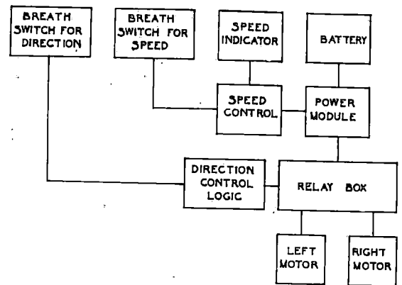
FIGURE 2. Schematic Diagram of Breath Operated Controls for Proportional Speed Motorized Chair.
