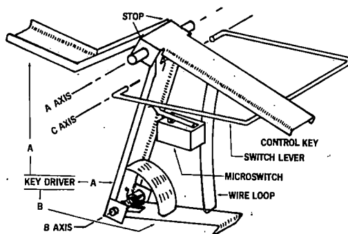
Figure 3. Control key and key driver combination.
