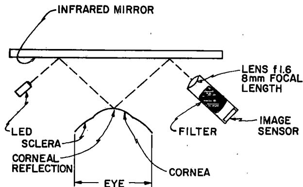
Figure 3. Sketch of Optics Used in Ocular Transducer.
