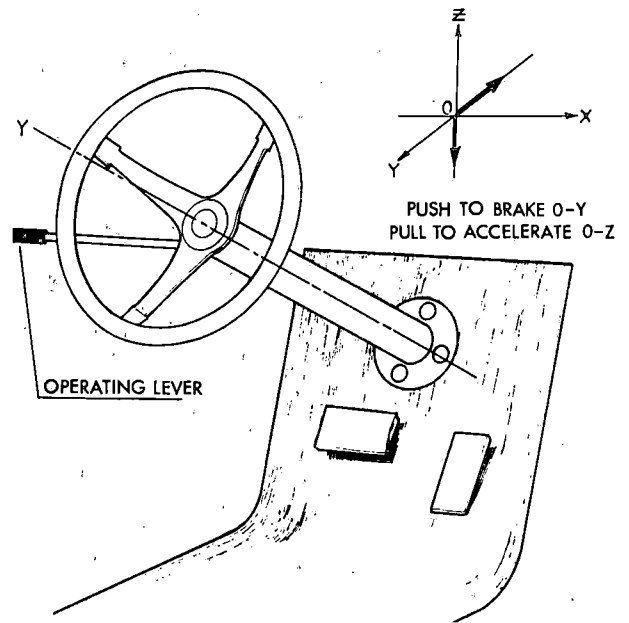
Fig. 2 Push-right angle pull type control system
