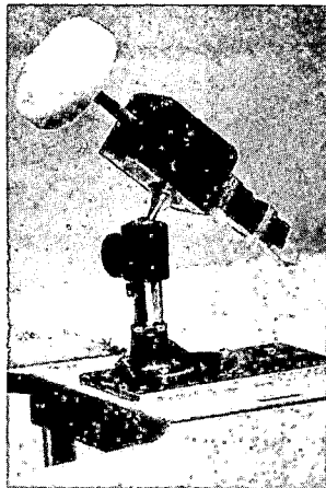
Fig. 5- Chin Switch Controller-on/off x/y axis device. Selector is activated by pushing inward.
