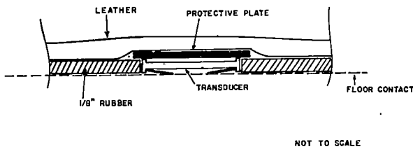
Figure 7 Sandal Mounting Arrangement of Transducer
