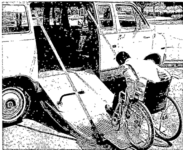
Fig. 8 Dodge Sportsman van, including integral wheelchair entry-exit system (Royce International, Englewood, Colorado)
