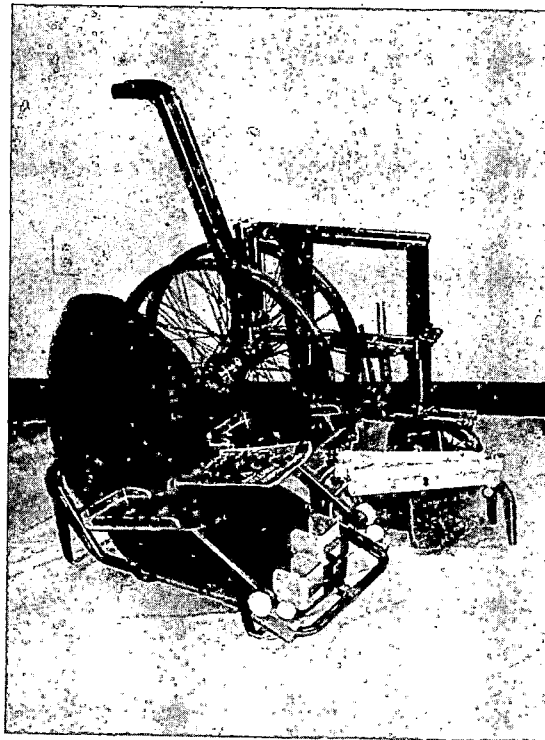
Figure 7, molded seat detached from wheelchair base.
