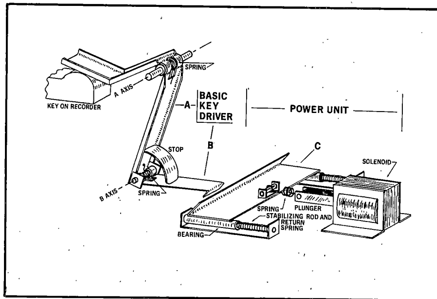
Figure 1. The power unit and basic key driver
