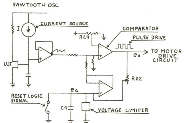
Figure 5. Diagram, acceleration limiter circuit
