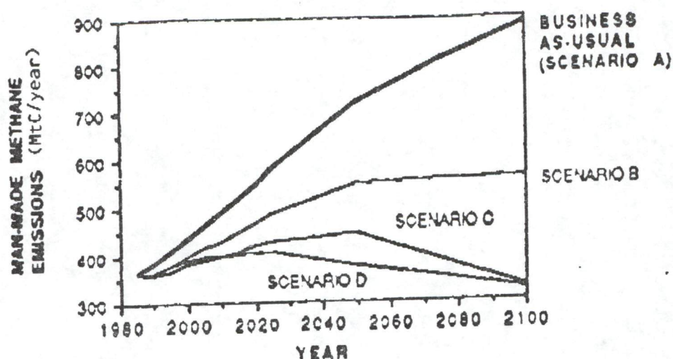
Figure 2. Projected Man-Made Methane Emissions (Million tonnes carbon per year)
