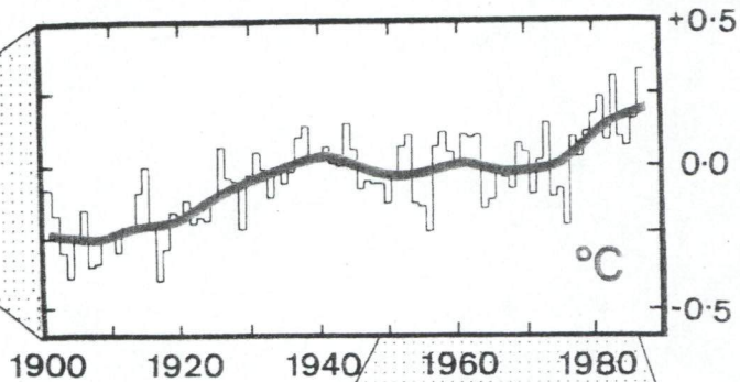
Global surface air temperature
