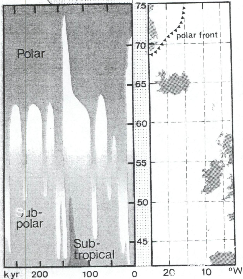
Plankton abundance in the N E Atlantic
