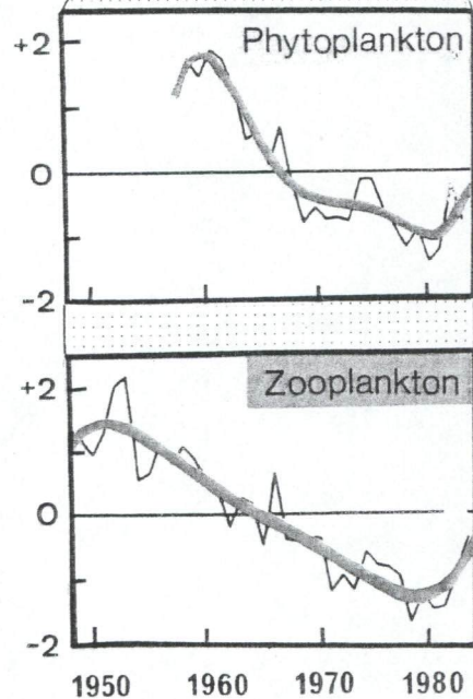
Plankton abundance in the N E Atlantic
