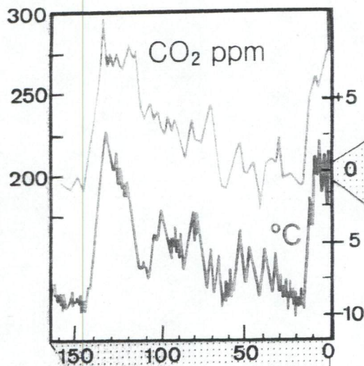
Global surface air temperature
