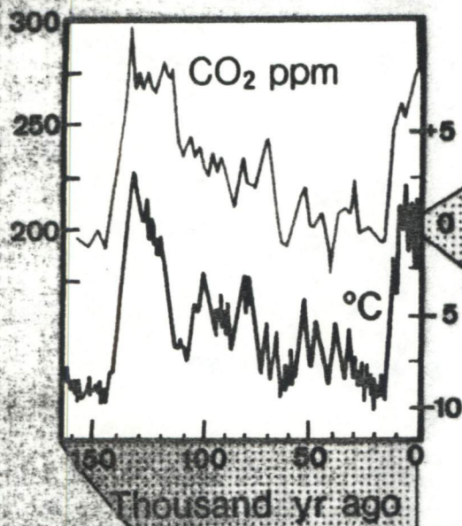
Global surface air temperature
