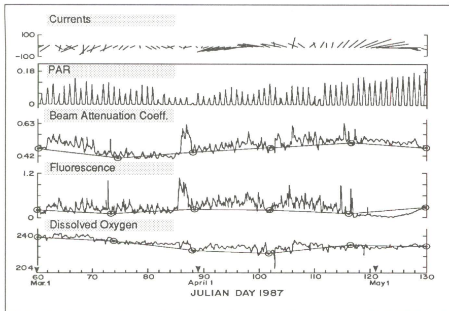
Fig. 2 Time series of daily averaged vector currents (in cm/sec) and two-hour filtered PAR (in \times 10^{21} quanta/ \text{m}^2/\text{sec} ), beam attenuation coefficient (in 1/\text{m} ), chlorophyll fluorescence (in \mu\text{g chl-a}/\text{l} ) and dissolved oxygen (in \mu\text{M} ) taken from the 20 MVMS during the first deployment of the Biowatt mooring. Currents were very low as the springtime stratification (not shown) began on JD 86 (mixed layer shoaling from greater than 160m to about 30m). A major transient springtime bloom shows in the beam attenuation coefficient and chlorophyll fluorescence time series. Bi-weekly subsampled data are indicated with circles connected by straight lines. The undersampling problem of previous data sets is apparent.
