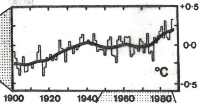
Global surface air temperature
