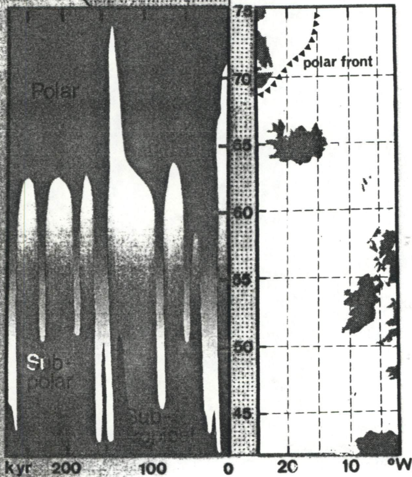
N-S migration of polar and subpolar waters: benthic core data in vicinity of 20°W
